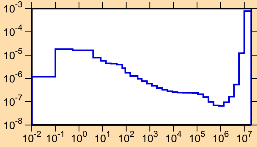
\sigma vs. E for ^{248}\text{Es}(n,\alpha)
