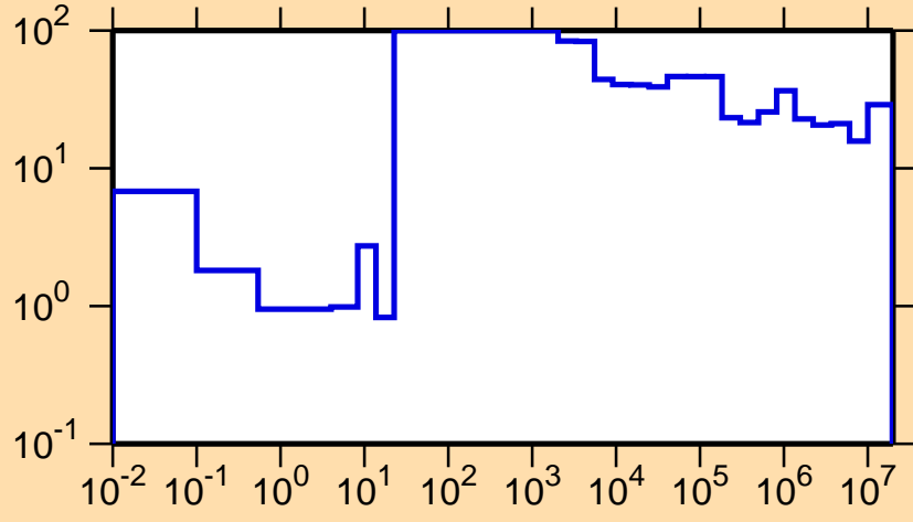
\Delta\sigma/\sigma vs. E for ^{248}\text{Es}(n,el.)
