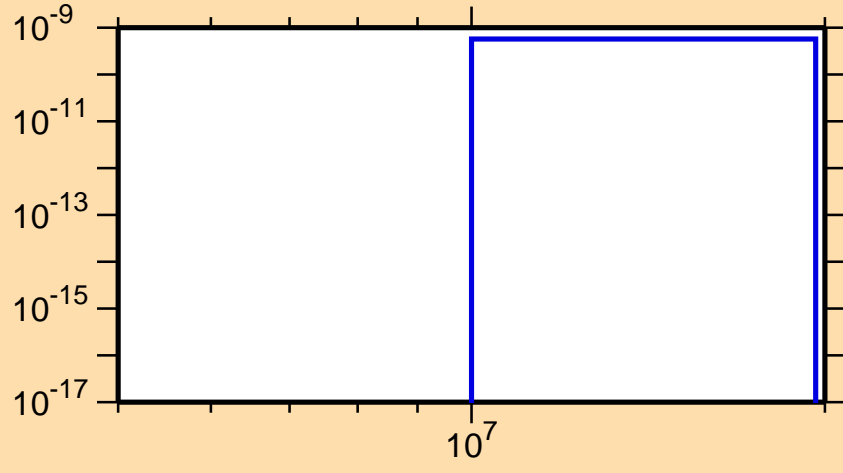
\sigma vs. E for ^{248}\text{Es}(n,\text{He3})
