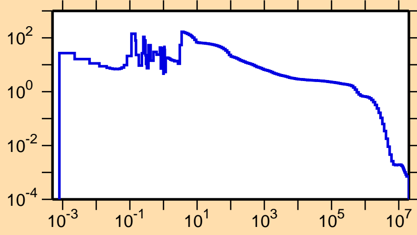
\sigma vs. E for ^{249}\text{Es}(n,\gamma)
