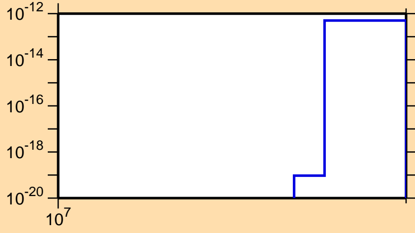
\sigma vs. E for ^{249}\text{Es} (mt 11)
