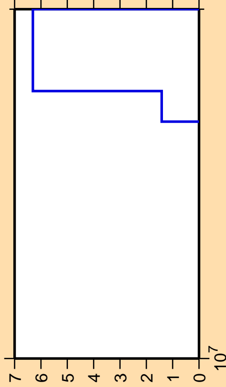
\Delta\sigma/\sigma vs. E for ^{249}\text{Es} (mt 45)
