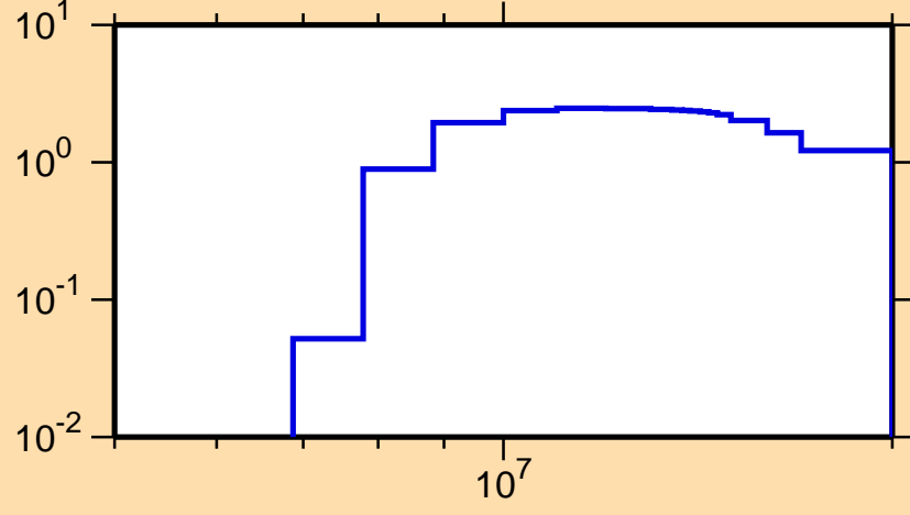
\sigma vs. E for ^{249}\text{Es}(n,2n)
