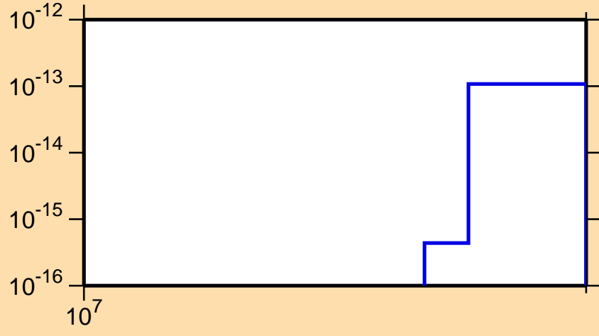
\sigma vs. E for ^{249}\text{Es} (mt 34)
