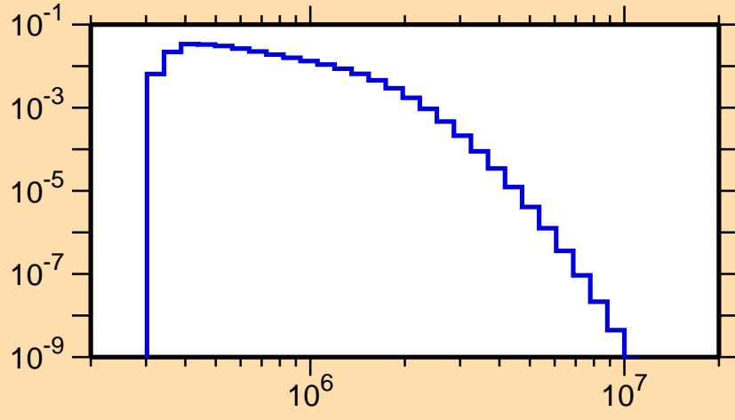
\sigma vs. E for ^{250}\text{Es}(n,n_2)
