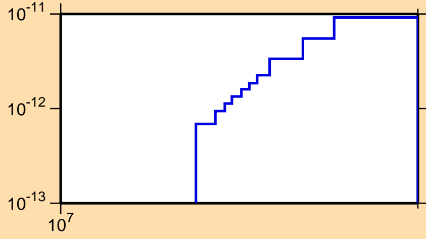
\sigma vs. E for ^{250}\text{Es}(n,p\alpha)
