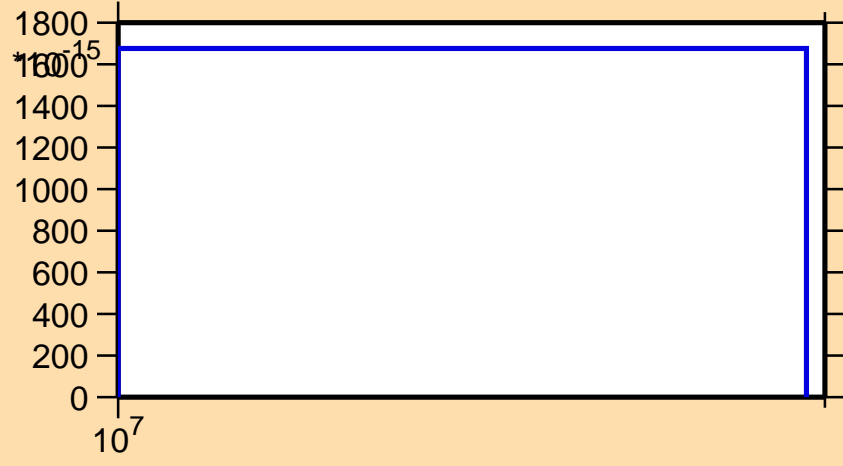
\sigma vs. E for ^{250}\text{Es}(n,p\alpha)
