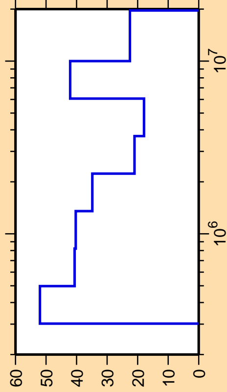
\Delta\sigma/\sigma vs. E for ^{250}\text{Es}(n,n\text{cont.})
