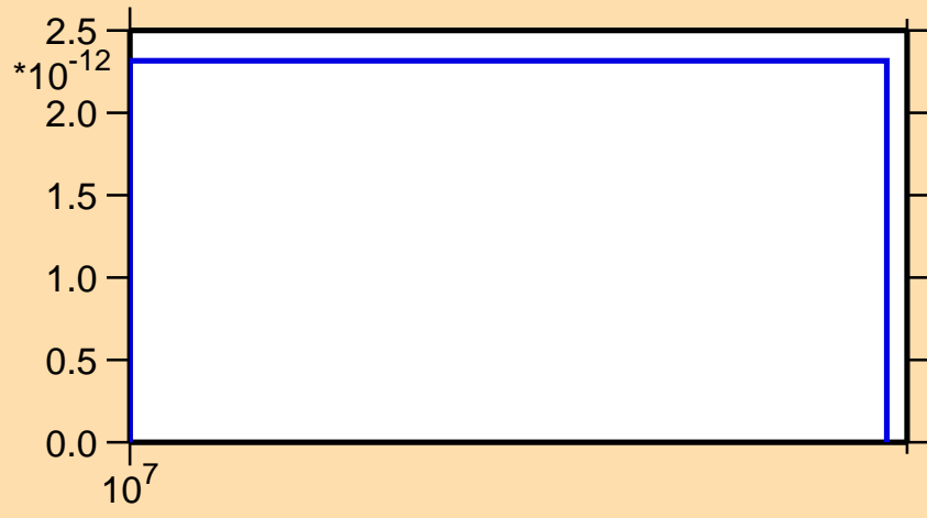
\sigma vs. E for ^{250}\text{Es}(n,3n\alpha)
