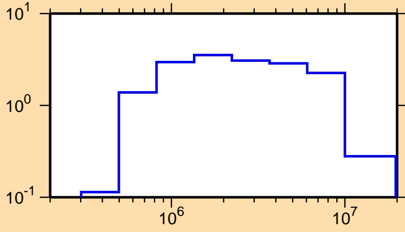
\sigma vs. E for ^{250}\text{Es}(n,n\text{cont.})
