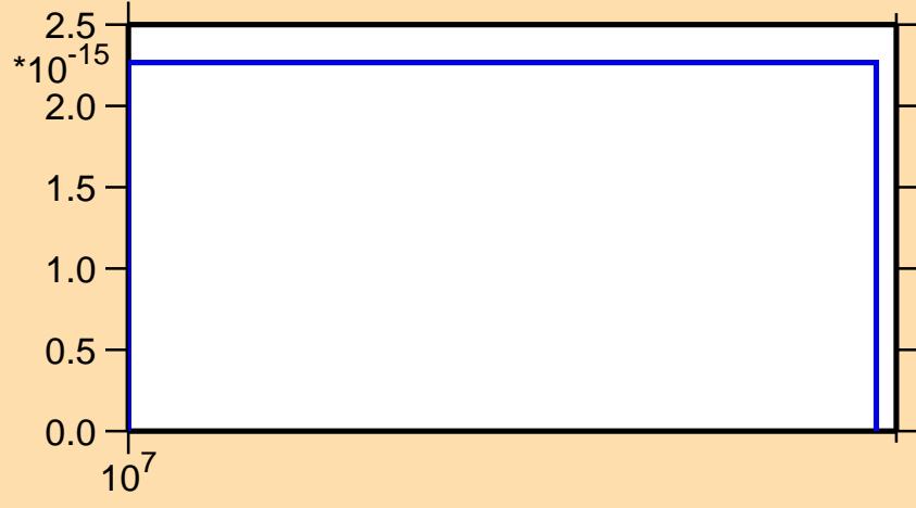
\sigma vs. E for ^{250}\text{Es} (mt 34)
