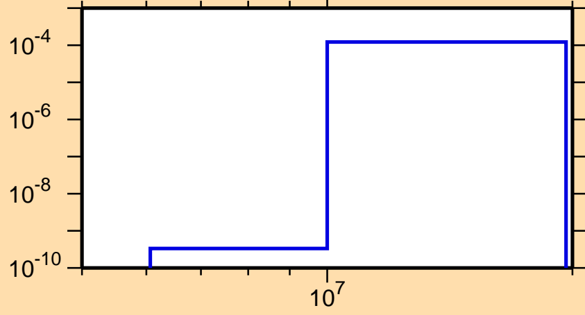
\sigma vs. E for ^{250}\text{Es}(n,t)
