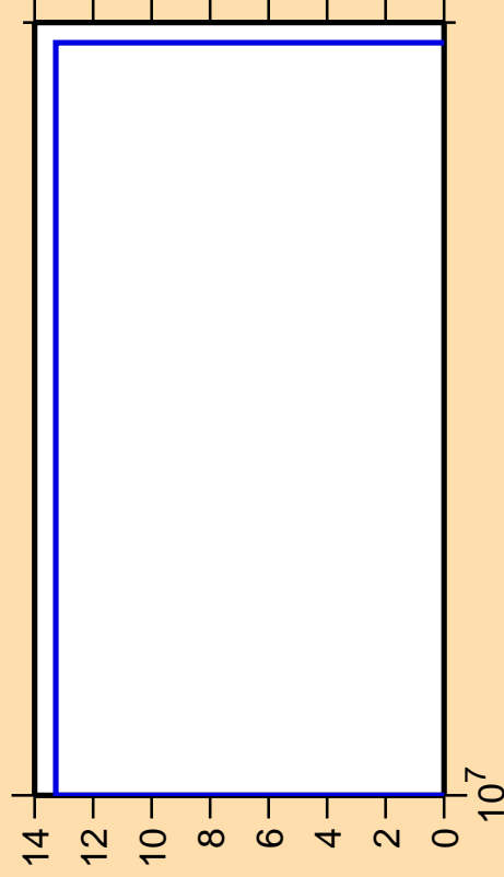
\Delta\sigma/\sigma vs. E for ^{250}\text{Es}(n,p\alpha)
