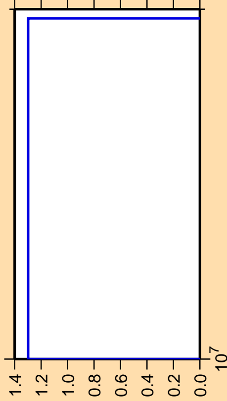
\Delta\sigma/\sigma vs. E for ^{250}\text{Es}(n,3n\alpha)
