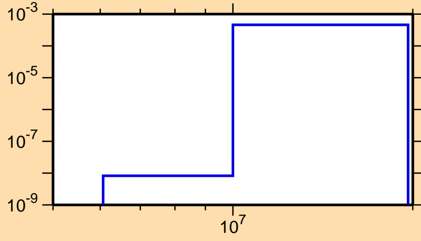
\sigma vs. E for ^{250}\text{Es}(n,d)
