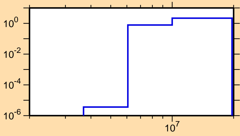
\sigma vs. E for ^{250}\text{Es}(n,2n)
