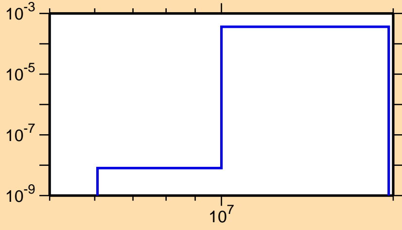
\sigma vs. E for ^{250}\text{Es}(n,np)
