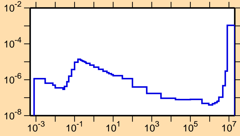
\sigma vs. E for ^{250}\text{Es}(n,\alpha)
