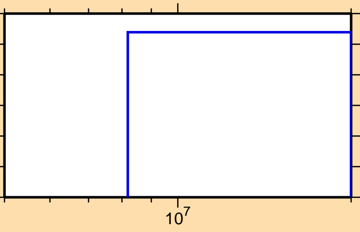
\sigma vs. E for ^{250}\text{Es}(n,p\alpha)
