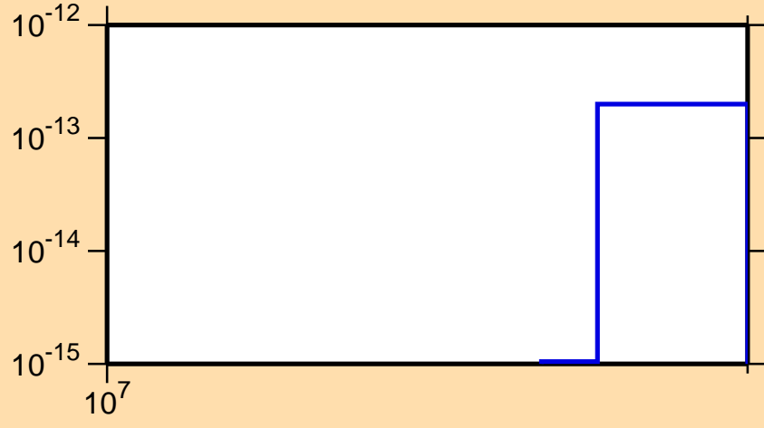
\sigma vs. E for ^{252}\text{Es} (mt 34)
