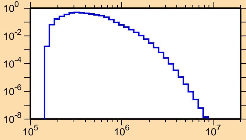
\sigma vs. E for ^{252}\text{Es}(n,n_2)
