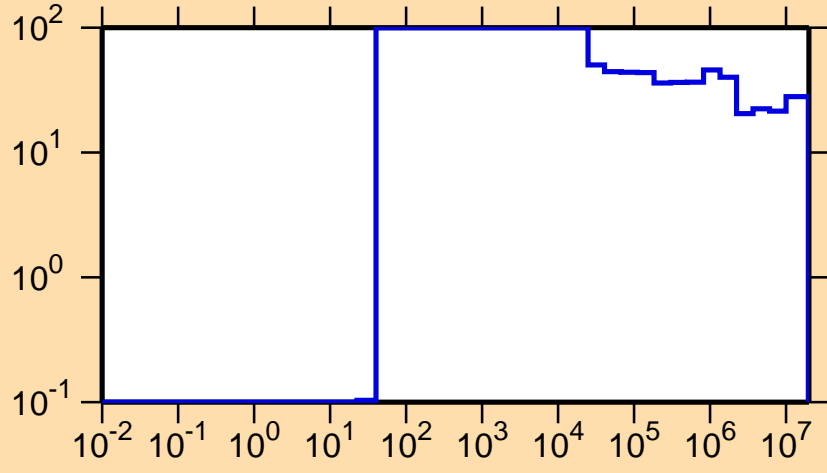
\Delta\sigma/\sigma vs. E for ^{252}\text{Es}(n,el.)
