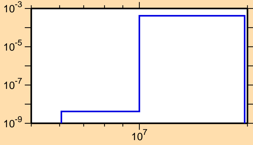
\sigma vs. E for ^{252}\text{Es}(n,d)
