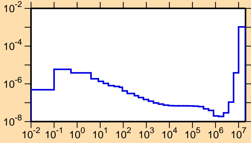
\sigma vs. E for ^{252}\text{Es}(n,\alpha)
