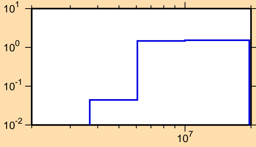
\sigma vs. E for ^{252}\text{Es}(n,2n)
