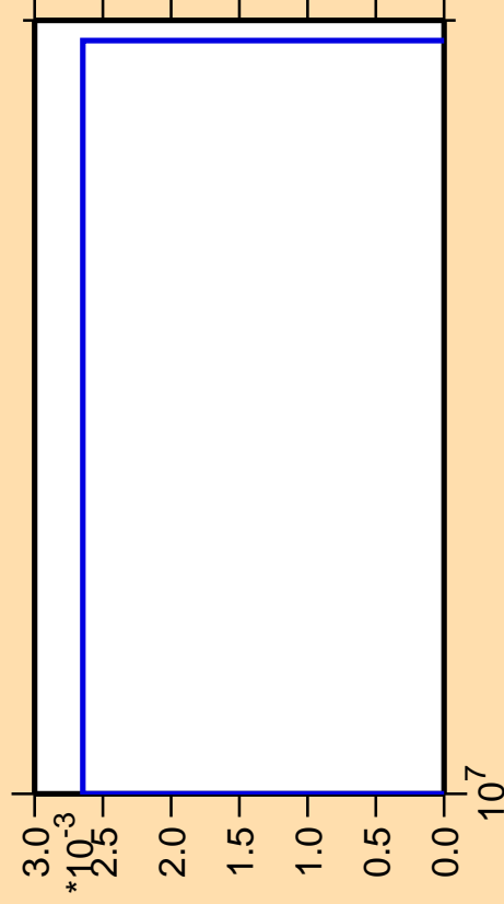
\Delta\sigma/\sigma vs. E for ^{252}\text{Es} (mt 42)
