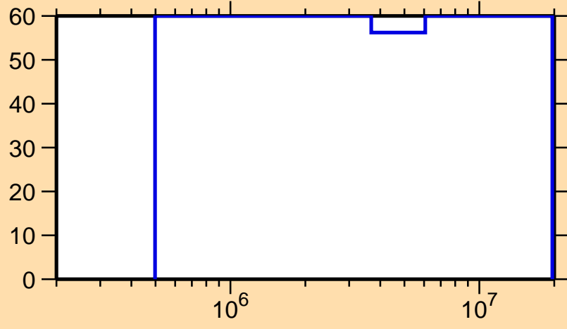
\Delta\sigma/\sigma vs. E for ^{252}\text{Es}(n,n\text{cont.})
