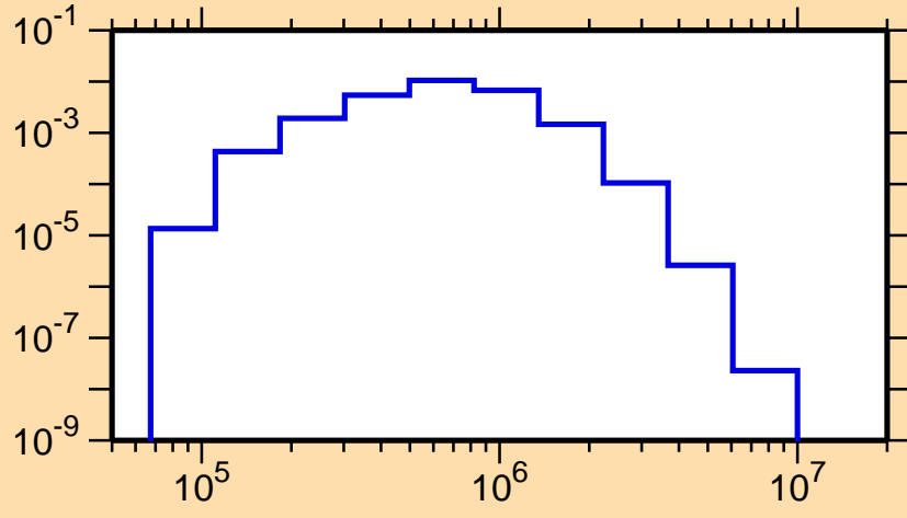
\sigma vs. E for ^{252}\text{Es}(n,n_1)
