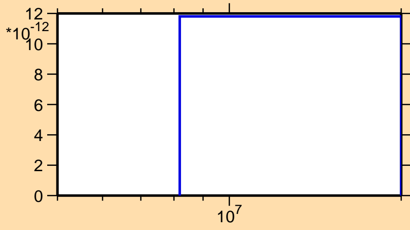
\sigma vs. E for ^{252}\text{Es}(n,\text{He3})
