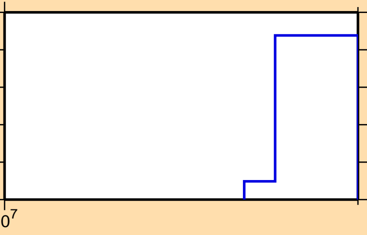
\sigma vs. E for ^{253}\text{Es}(n,3n\alpha)
