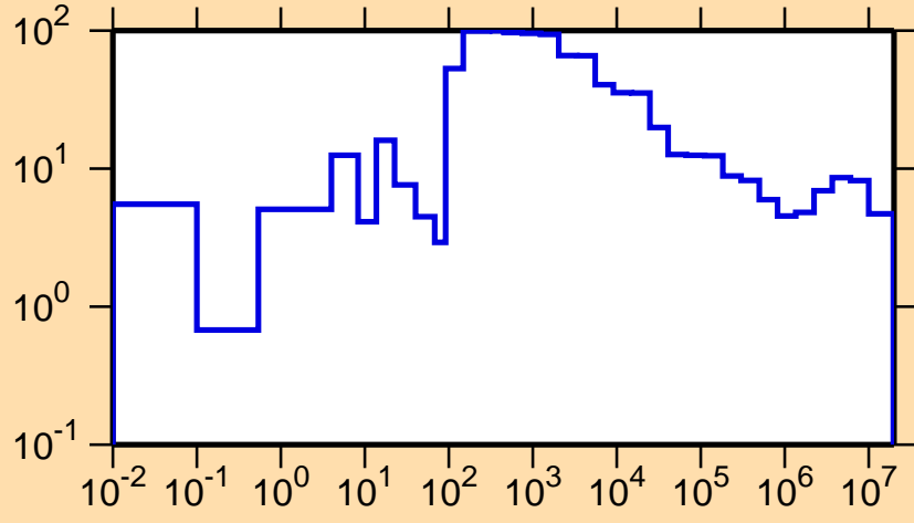
\Delta\sigma/\sigma vs. E for ^{253}\text{Es}(n,el.)
