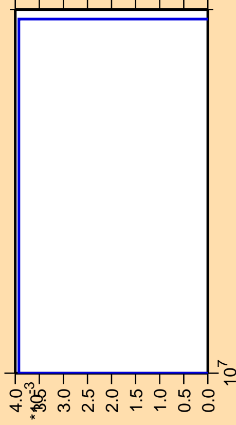
\Delta\sigma/\sigma vs. E for ^{253}\text{Es} (mt 42)
