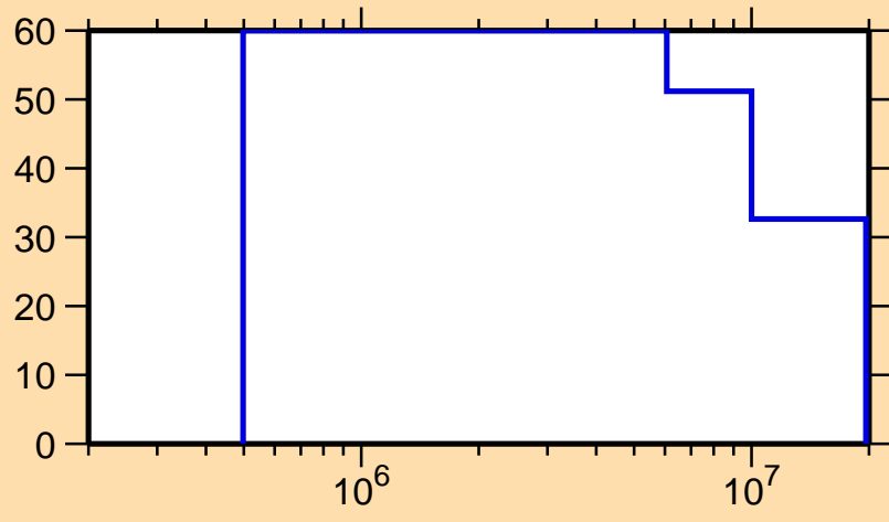
\Delta\sigma/\sigma vs. E for ^{253}\text{Es}(n,n\text{cont.})
