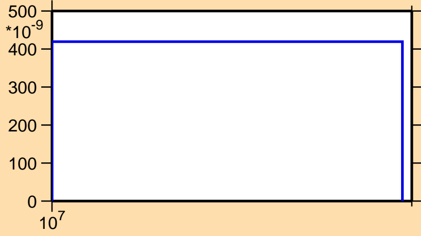
\sigma vs. E for ^{253}\text{Es}(n,nt)
