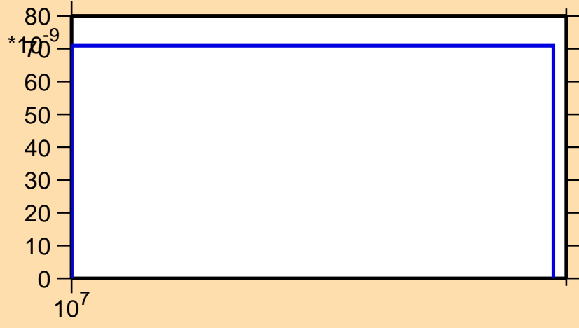
\sigma vs. E for ^{253}\text{Es}(n,\text{nd})
