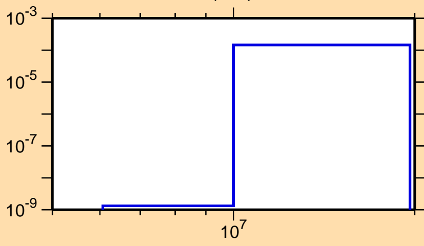
\sigma vs. E for ^{253}\text{Es}(n,d)
