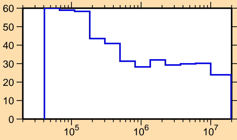
\Delta\sigma/\sigma vs. E for ^{253}\text{Es}(n,n_1)
