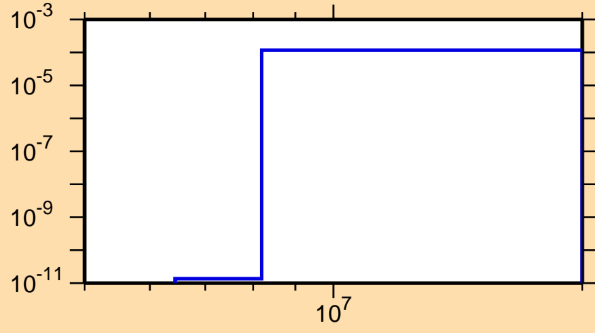
\sigma vs. E for ^{253}\text{Es}(n,d)
