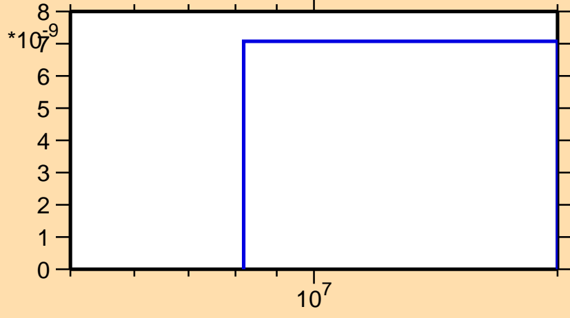
\sigma vs. E for ^{253}\text{Es}(n,2np)
