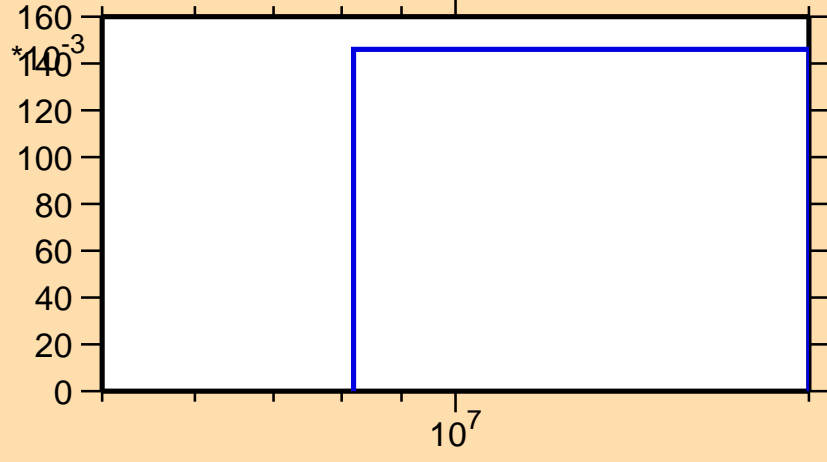
\sigma vs. E for ^{253}\text{Es}(n,3n)
