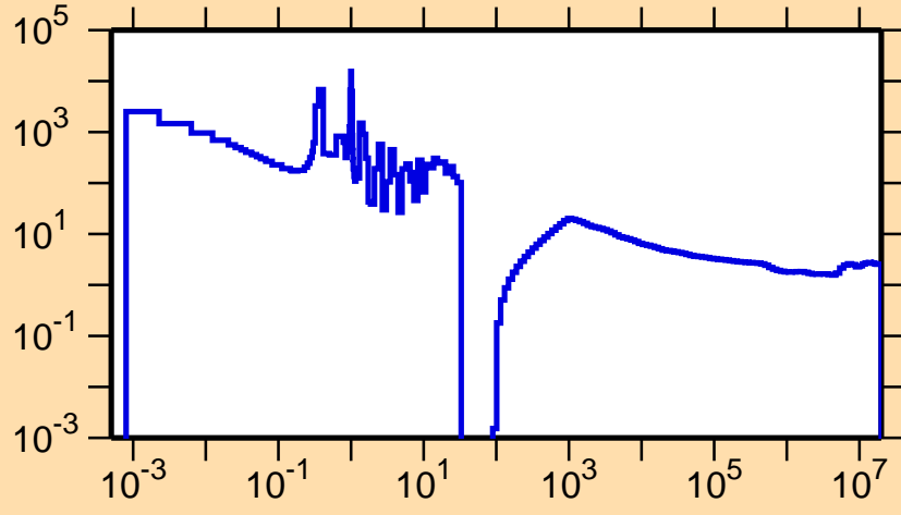
\sigma vs. E for ^{254}\text{Es}(n,f)
