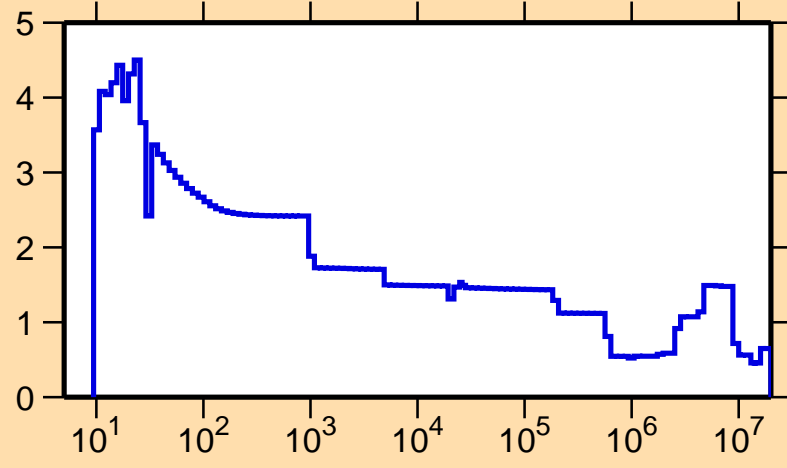
\Delta\sigma/\sigma vs. E for ^{254}\text{Es}(n,\text{tot.})
