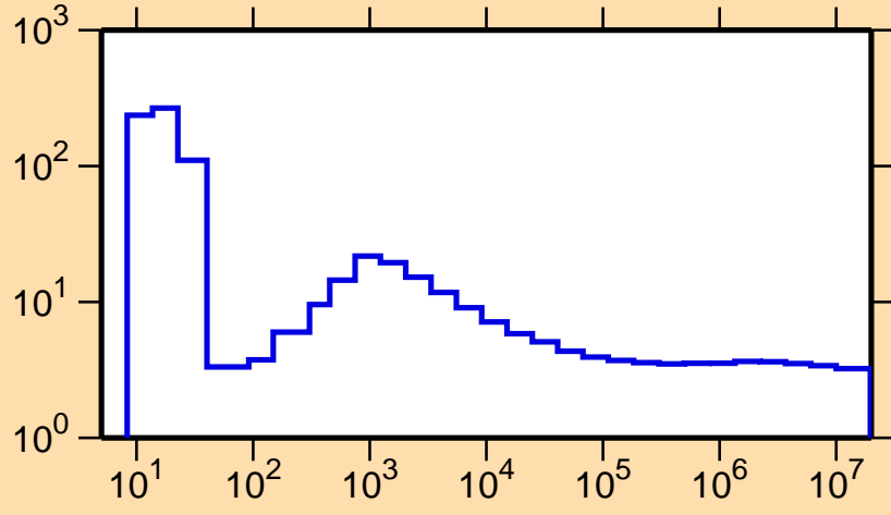
\sigma vs. E for ^{254}\text{Es}(n,\text{nonel.})
