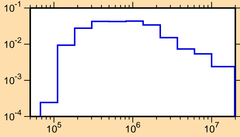
\sigma vs. E for ^{254}\text{Es}(n,n_2)
