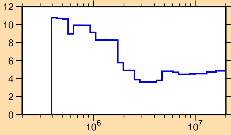
\Delta\sigma/\sigma vs. E for ^{254}\text{Es}(n,\text{nonel.})
