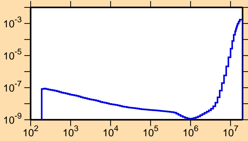
\sigma vs. E for ^{254}\text{Es}(n, \alpha)
