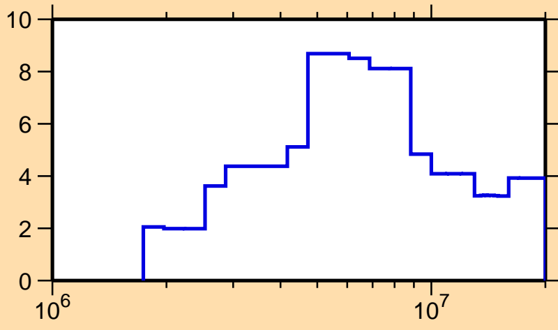
\Delta\sigma/\sigma vs. E for ^{254}\text{Es}(n,\text{tot.})
