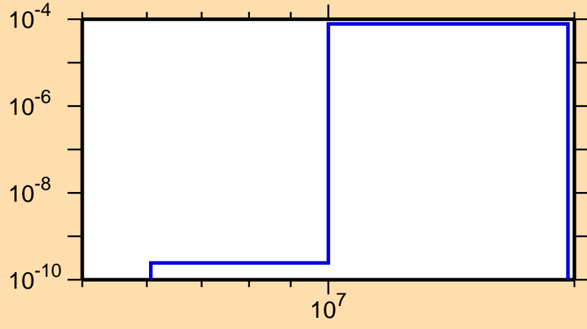
\sigma vs. E for ^{254}\text{Es}(n,t)
