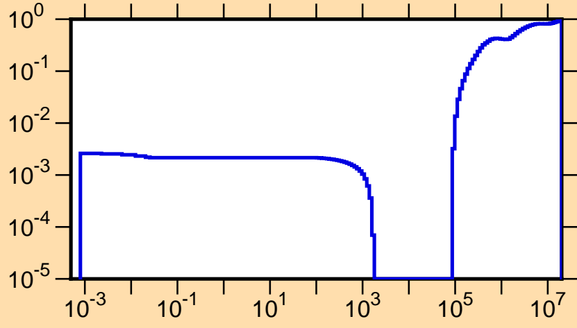
\mu vs. E for ^{255}\text{Es}(\text{mt251})
