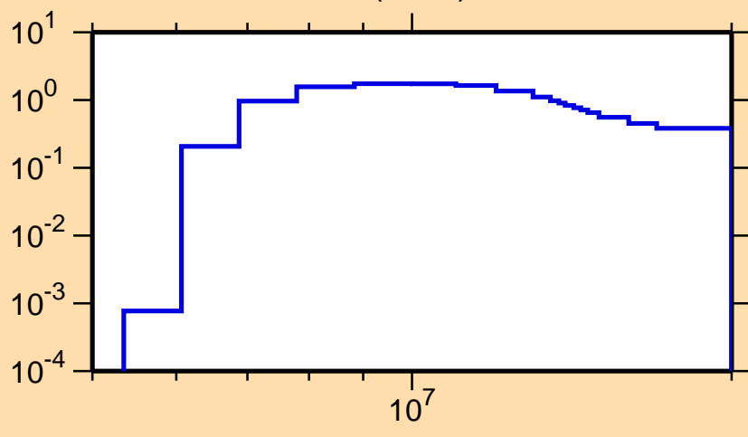
\sigma vs. E for ^{255}\text{Es}(n,2n)
