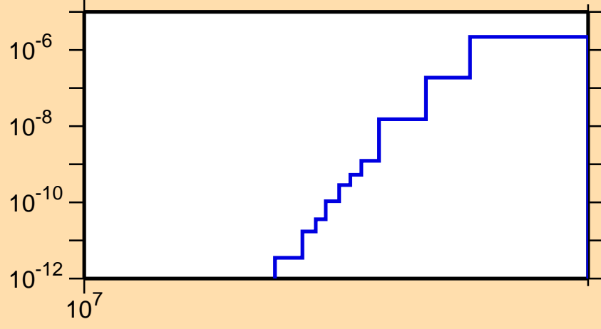
\sigma vs. E for ^{255}\text{Es}(n,nd)
