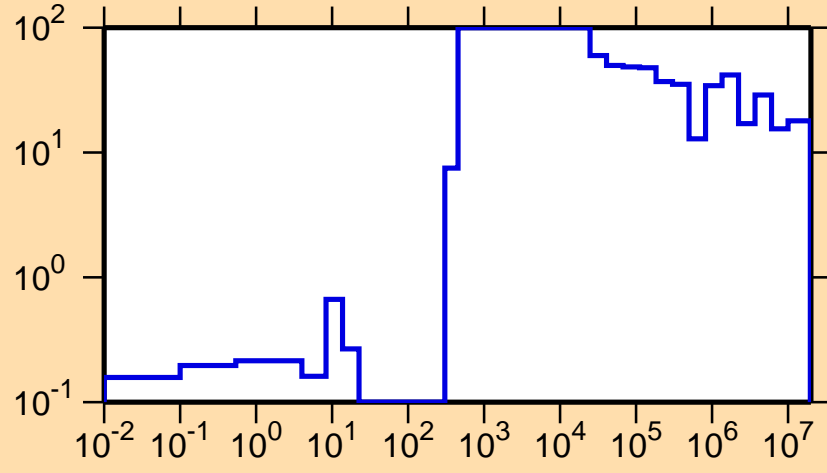
\Delta\sigma/\sigma vs. E for ^{255}\text{Es}(n,el.)
