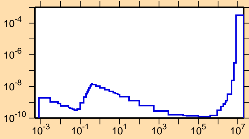
\sigma vs. E for ^{255}\text{Es}(n,\alpha)
