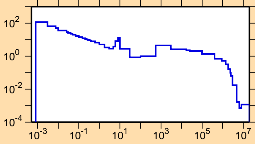
\sigma vs. E for ^{255}\text{Es}(n,\gamma)
