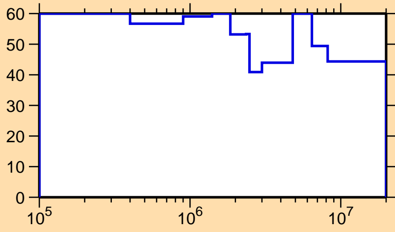
\Delta\sigma/\sigma vs. E for ^{255}\text{Es}(n,n_1)
