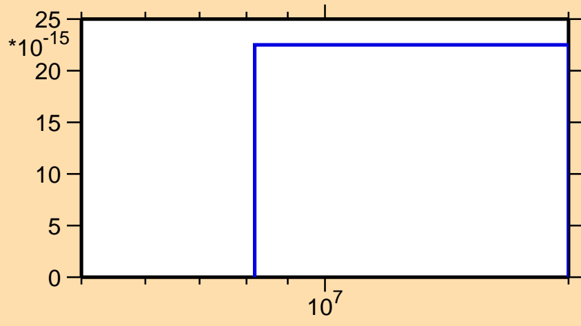
\sigma vs. E for ^{255}\text{Es} (mt 42)
