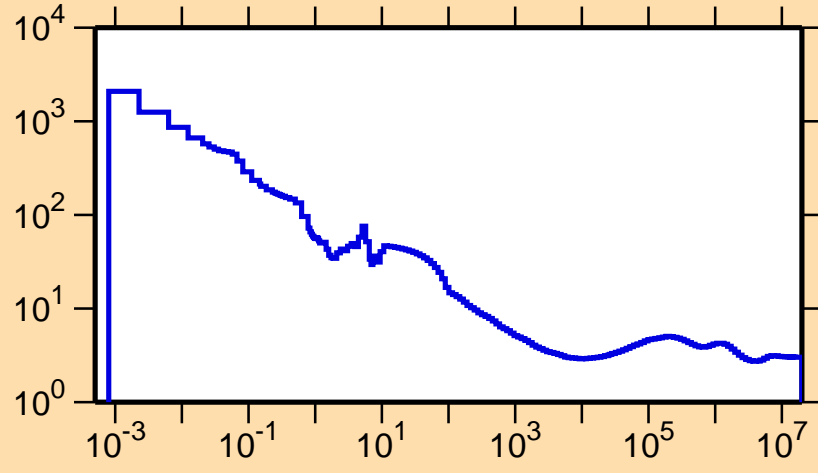
\sigma vs. E for ^{256}\text{Es}(n,\text{nonel.})
