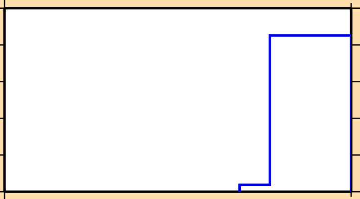
\sigma vs. E for ^{256}\text{Es} (mt 11)
