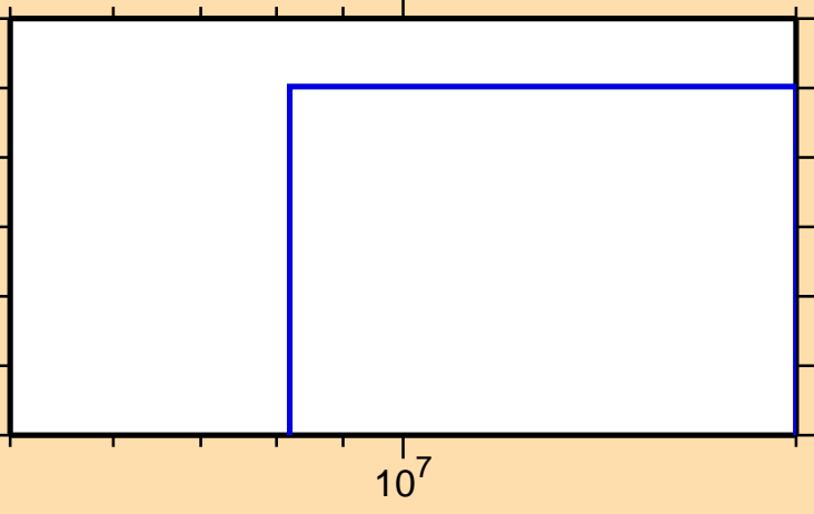
\sigma vs. E for ^{256}\text{Es}(n,2np)
