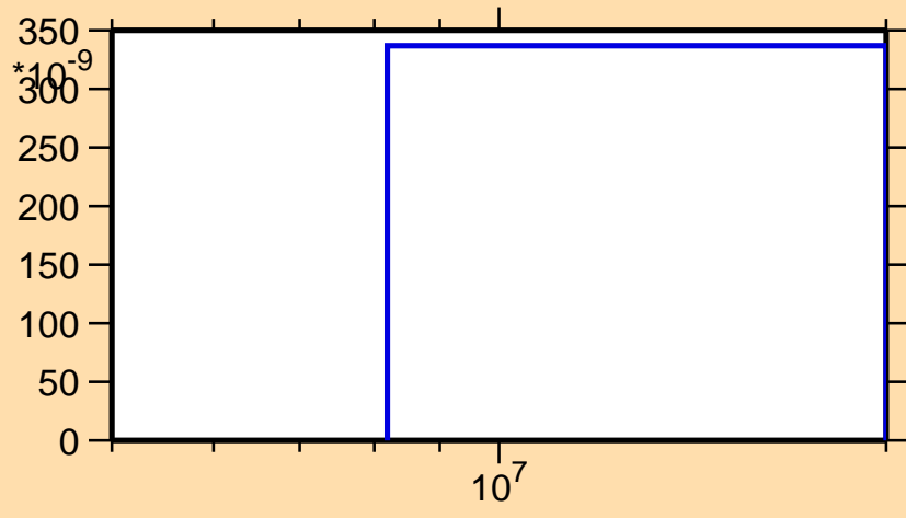
\sigma vs. E for ^{256}\text{Es}(n,nd)
