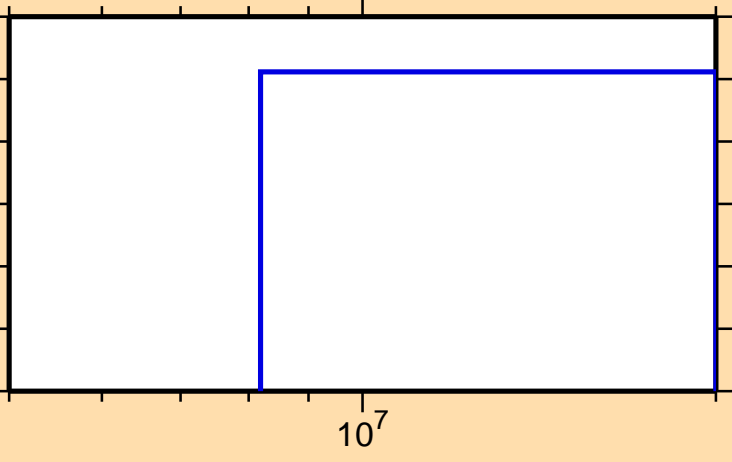
\sigma vs. E for ^{256}\text{Es}(n,\text{He3})
