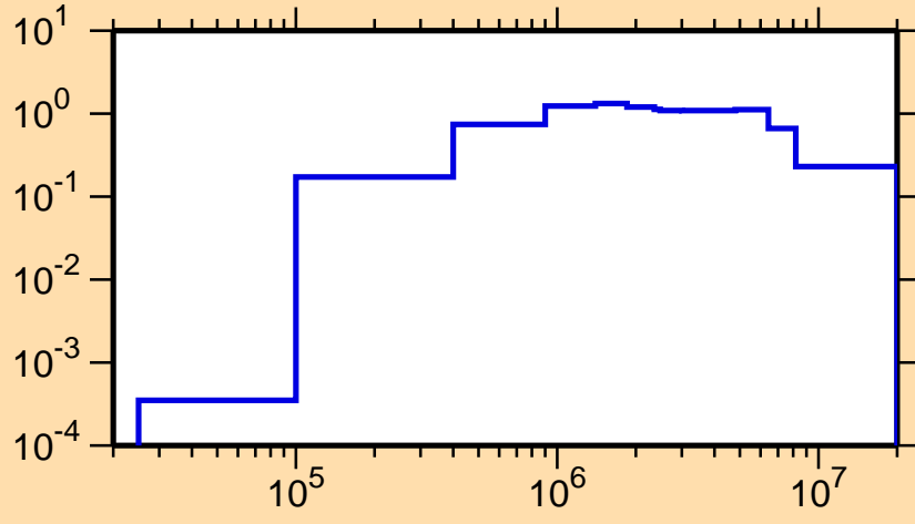
\sigma vs. E for ^{256}\text{Es}(n,n\text{cont.})
