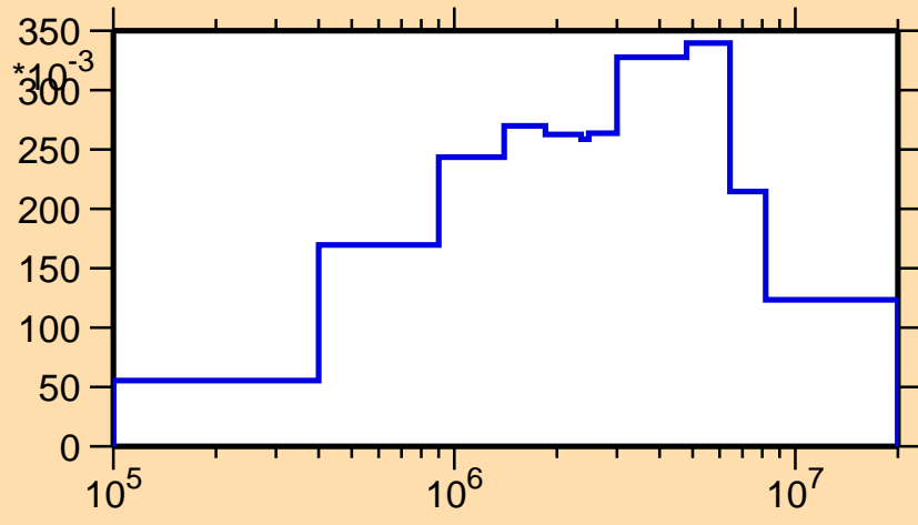
\sigma vs. E for ^{257}\text{Es}(n,n\text{cont.})
