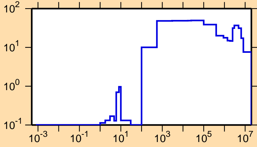
\Delta\sigma/\sigma vs. E for ^{257}\text{Es}(n,el.)
