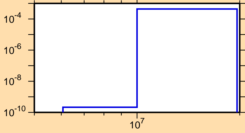
\sigma vs. E for ^{135}\text{Eu}(n,t)
