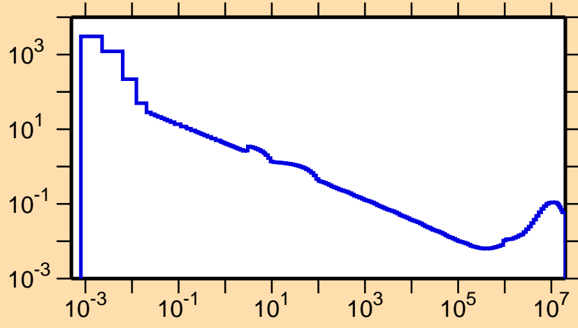
\sigma vs. E for ^{136}\text{Eu}(n,\alpha)
