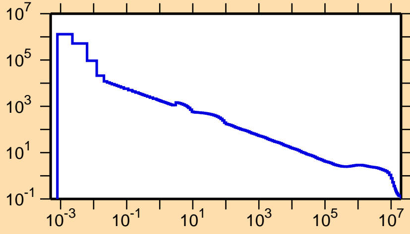
\sigma vs. E for ^{136}\text{Eu}(n,p)
