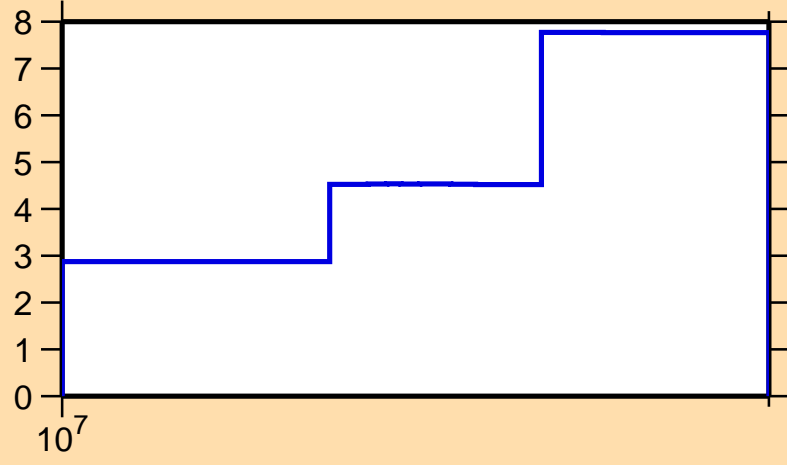
\Delta\sigma/\sigma vs. E for ^{136}\text{Eu}(n,\text{tot.})
