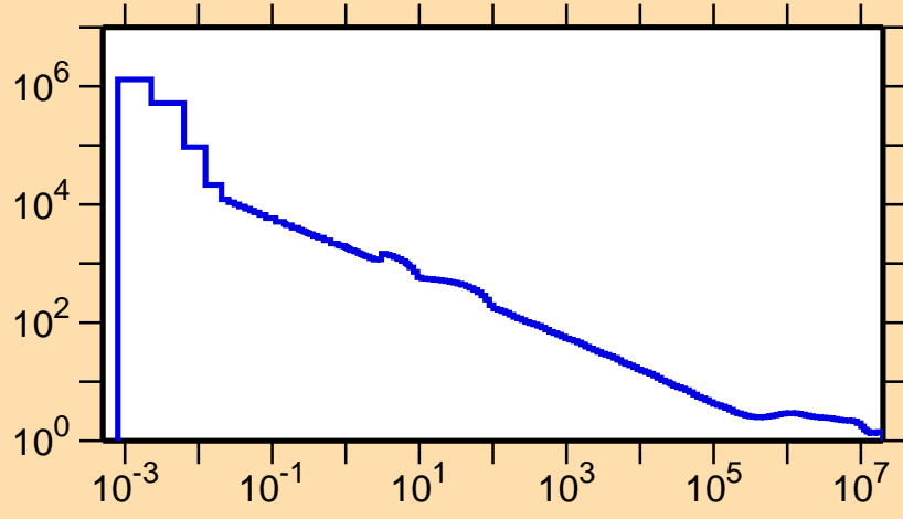
\sigma vs. E for ^{136}\text{Eu}(n,\text{nonel.})
