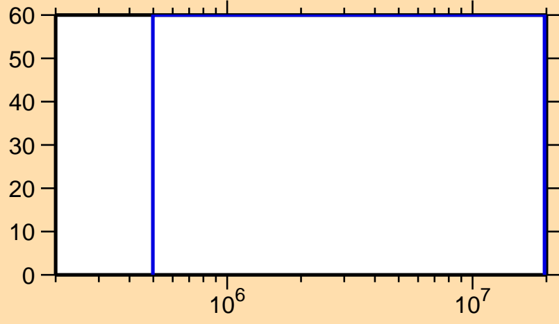
\Delta\sigma/\sigma vs. E for ^{136}\text{Eu}(n,n_1)
