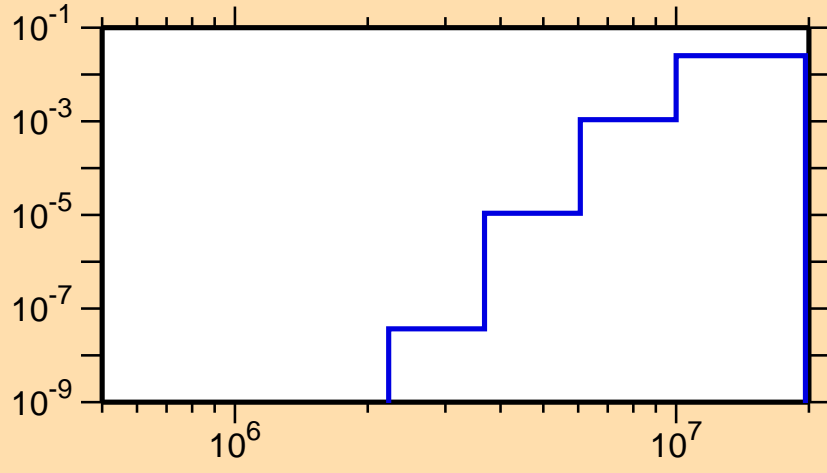
\sigma vs. E for ^{136}\text{Eu}(n,d)
