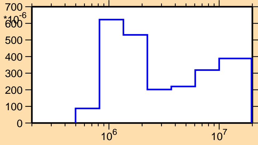
\sigma vs. E for ^{136}\text{Eu}(n,n_2)
