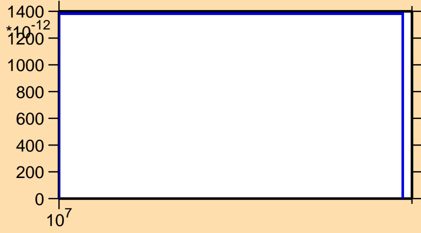
\sigma vs. E for ^{136}\text{Eu} (mt 34)
