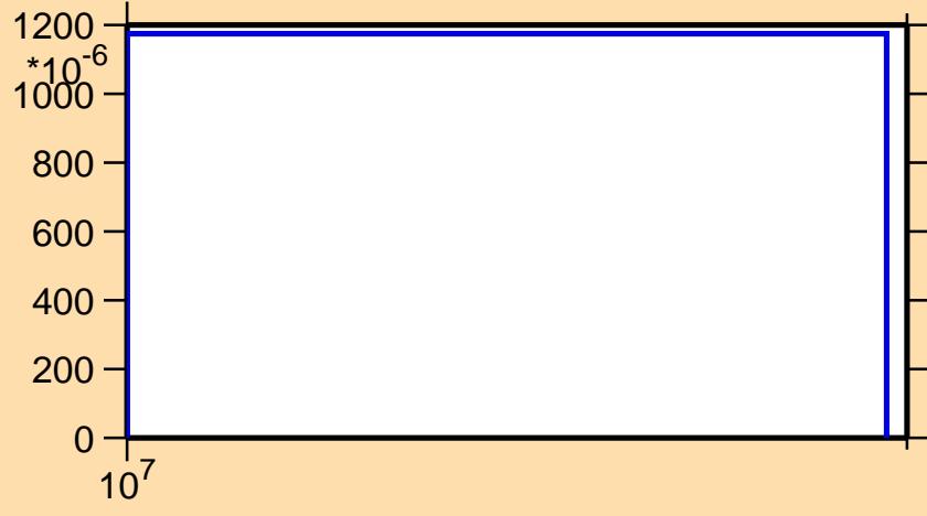
\sigma vs. E for ^{136}\text{Eu}(n,2n)
