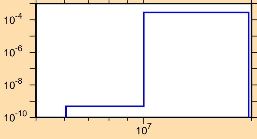
\sigma vs. E for ^{136}\text{Eu}(n,\text{pd})
