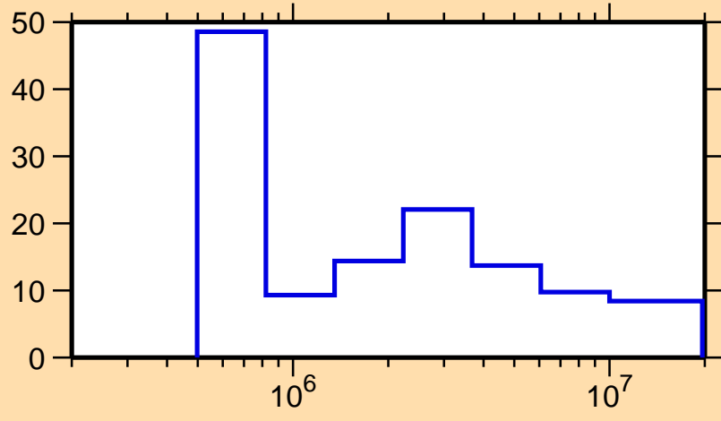
\Delta\sigma/\sigma vs. E for ^{136}\text{Eu}(n,\text{el.})
