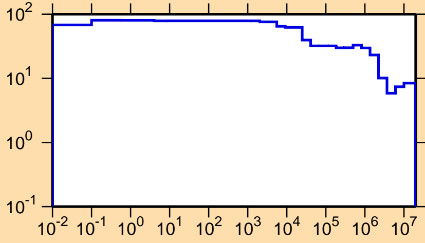
\Delta\sigma/\sigma vs. E for ^{136}\text{Eu}(n,\text{nonel.})
