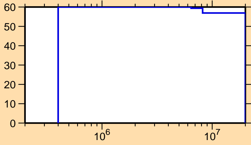
\Delta\sigma/\sigma vs. E for ^{136}\text{Eu}(n,n\text{cont.})
