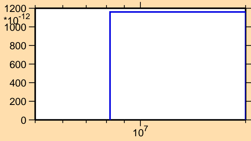
\sigma vs. E for ^{136}\text{Eu} (mt 34)
