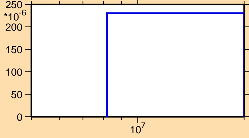
\sigma vs. E for ^{136}\text{Eu}(n,2np)
