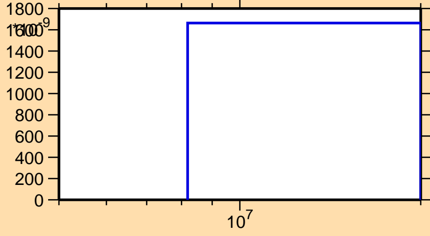
\sigma vs. E for ^{136}\text{Eu}(n,\text{nd})
