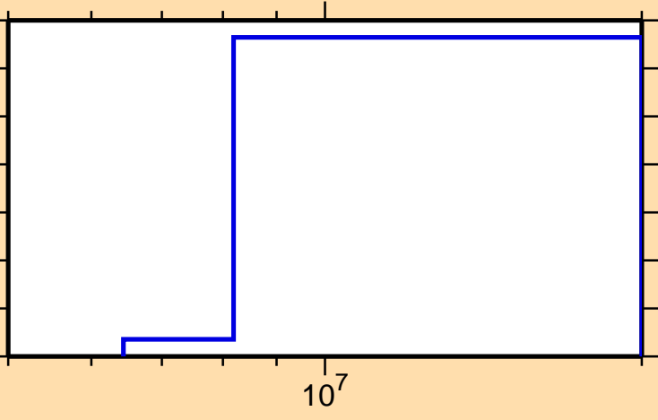
\sigma vs. E for ^{136}\text{Eu}(\text{mt117})
