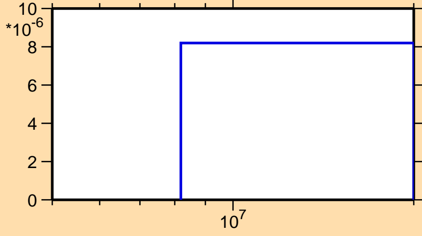
\sigma vs. E for ^{136}\text{Eu}(n,\text{pt})
