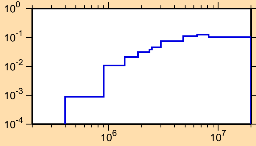
\sigma vs. E for ^{136}\text{Eu}(n,\text{inel.})
