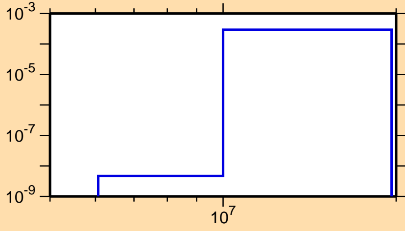
\sigma vs. E for ^{136}\text{Eu}(\text{mt } 45)
