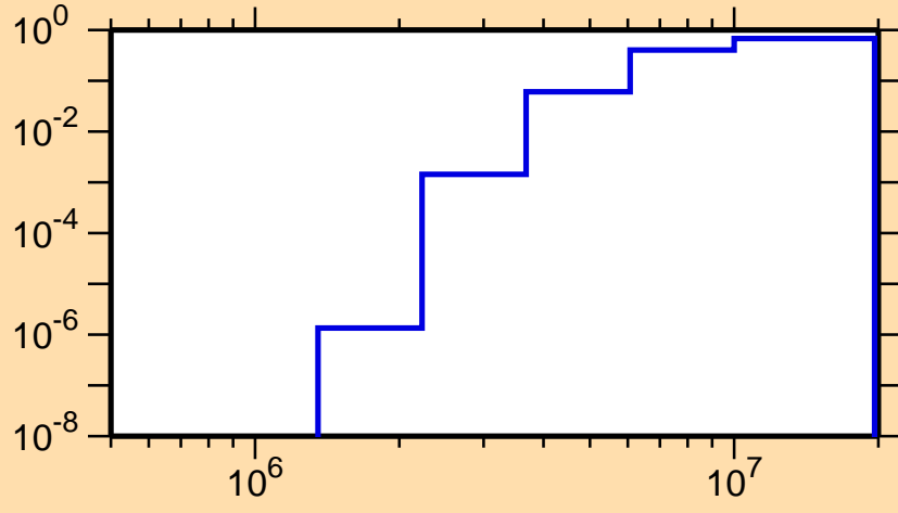
\sigma vs. E for ^{136}\text{Eu}(n,np)
