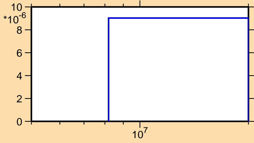
\sigma vs. E for ^{136}\text{Eu}(n,nd)
