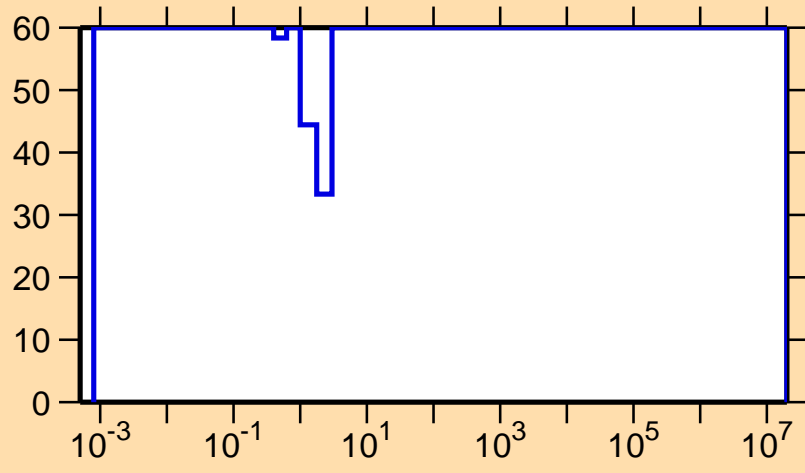
\Delta\sigma/\sigma vs. E for ^{136}\text{Eu}(n,\gamma)
