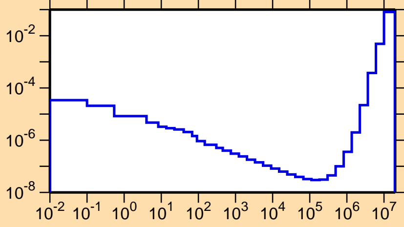
\sigma vs. E for ^{137}\text{Eu}(n,p\alpha)
