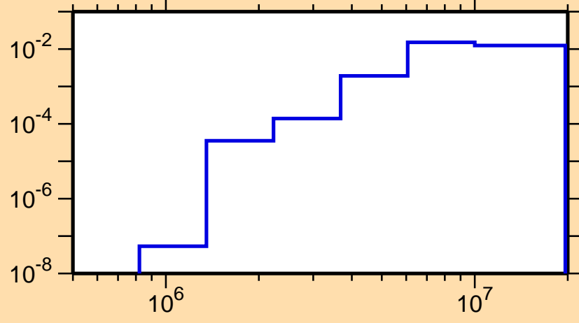
\sigma vs. E for ^{137}\text{Eu}(n,n\text{cont.})
