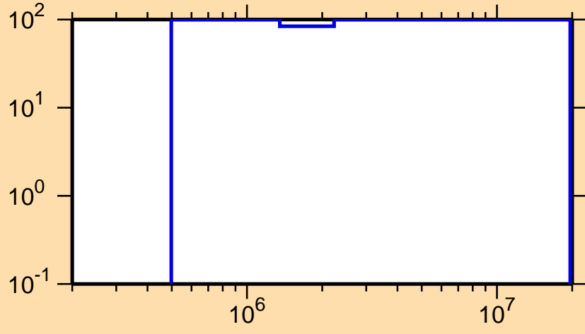
\Delta\sigma/\sigma vs. E for ^{137}\text{Eu}(n,n\text{cont.})
