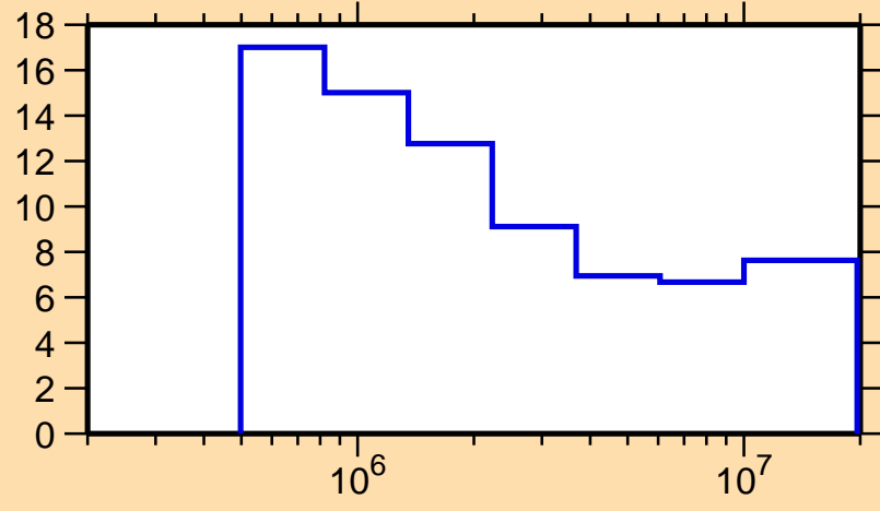
\Delta\sigma/\sigma vs. E for ^{137}\text{Eu}(n, el.)
