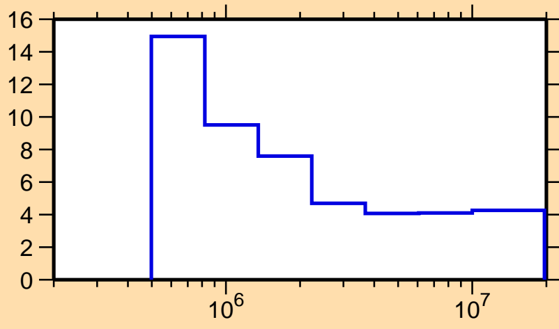
\Delta\sigma/\sigma vs. E for ^{137}\text{Eu}(n,\text{tot.})
