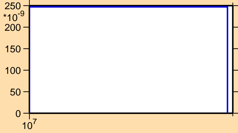
\sigma vs. E for ^{137}\text{Eu}(n,\text{nd})
