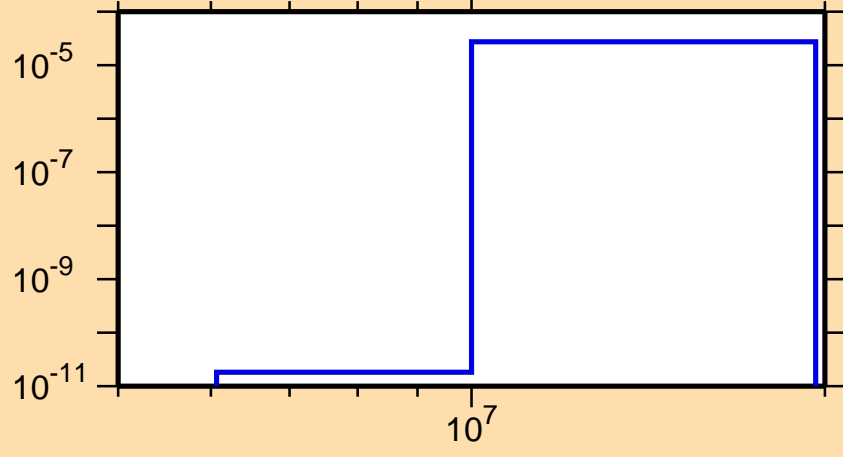
\sigma vs. E for ^{137}\text{Eu}(n,\text{pd})
