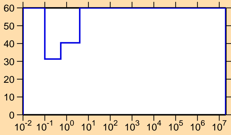
\Delta\sigma/\sigma vs. E for ^{137}\text{Eu}(n,\gamma)
