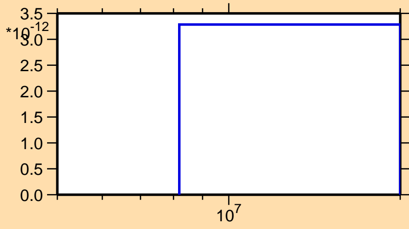
\sigma vs. E for ^{137}\text{Eu} (mt 34)
