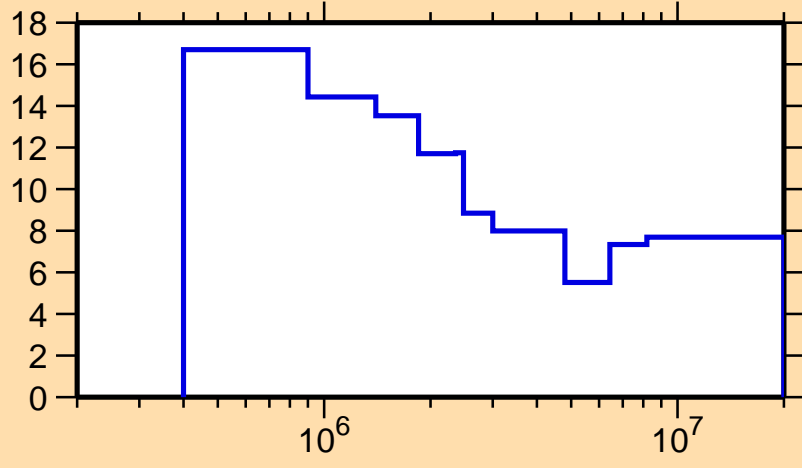
\Delta\sigma/\sigma vs. E for ^{137}\text{Eu}(n, el.)
