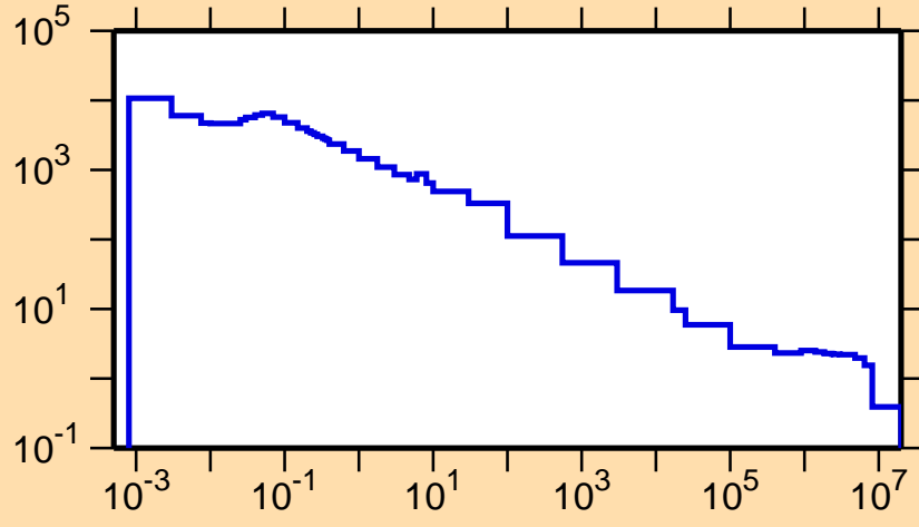
\sigma vs. E for ^{137}\text{Eu}(n,p)
