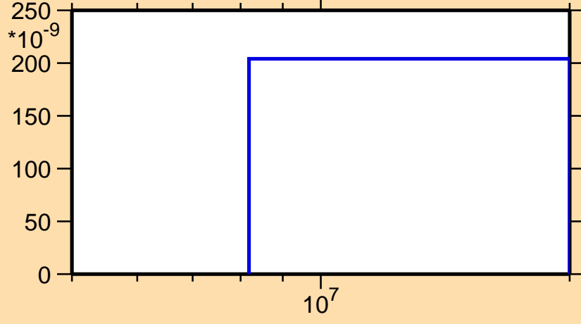
\sigma vs. E for ^{137}\text{Eu}(n,nd)
