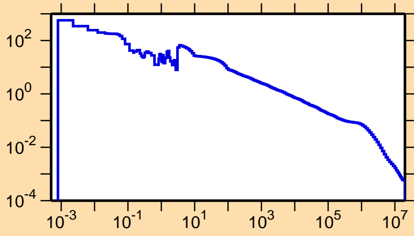
\sigma vs. E for ^{138}\text{Eu}(n,\gamma)
