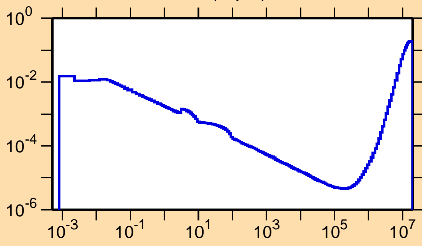
\sigma vs. E for ^{138}\text{Eu}(n,p\alpha)
