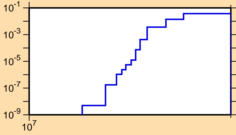
\sigma vs. E for ^{138}\text{Eu}(n,2np)
