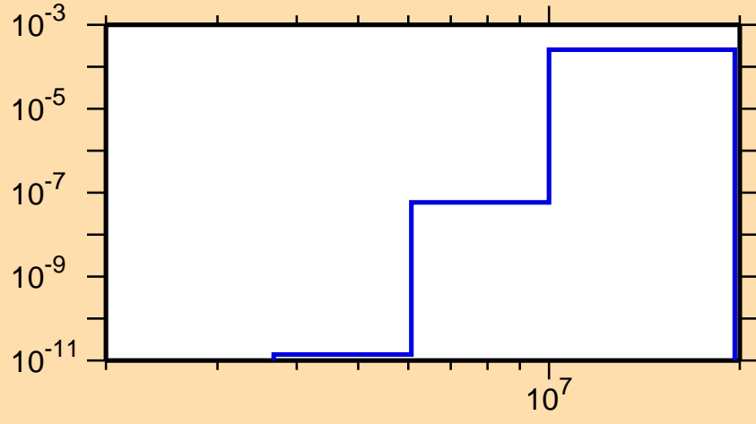
\sigma vs. E for ^{138}\text{Eu}(n,\text{He3})
