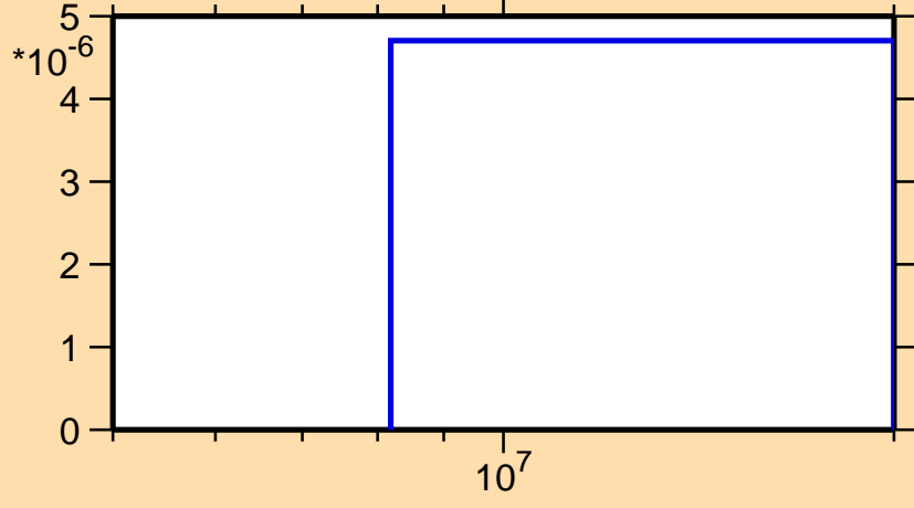
\sigma vs. E for ^{138}\text{Eu}(n,nd)
