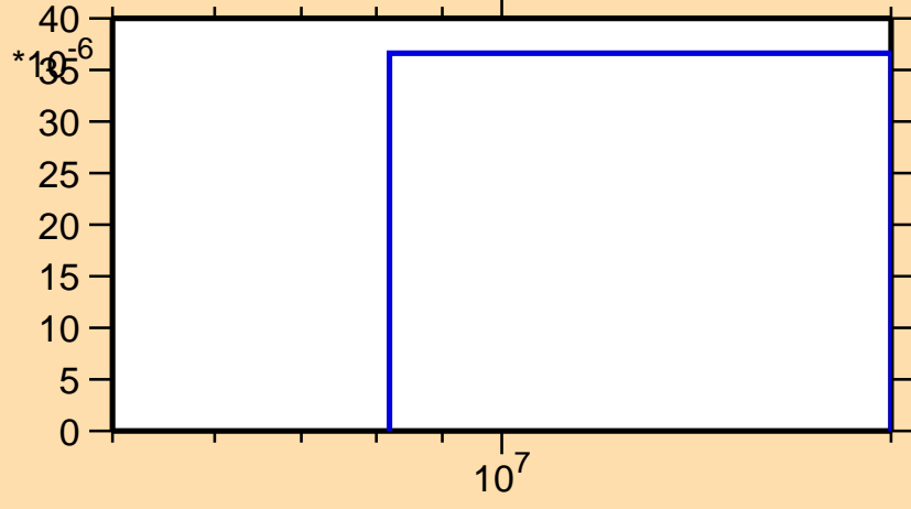
\sigma vs. E for ^{138}\text{Eu}(n,\text{pd})
