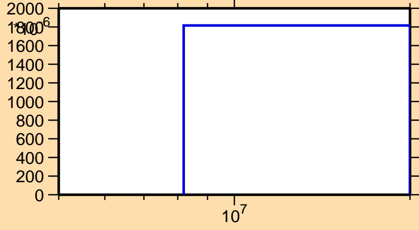
\sigma vs. E for ^{138}\text{Eu}(n,2n)
