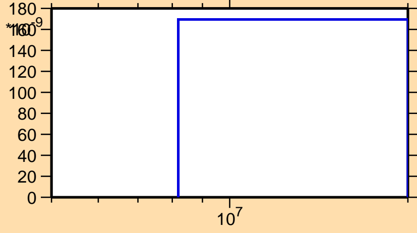
\sigma vs. E for ^{138}\text{Eu}(n,\text{pt})
