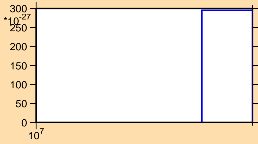
\sigma vs. E for ^{139}\text{Eu} (mt 11)
