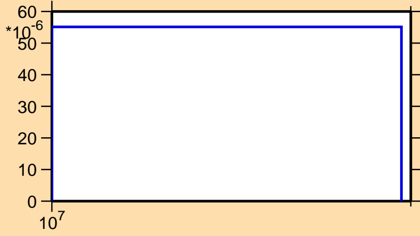
\sigma vs. E for ^{139}\text{Eu}(n,2np)
