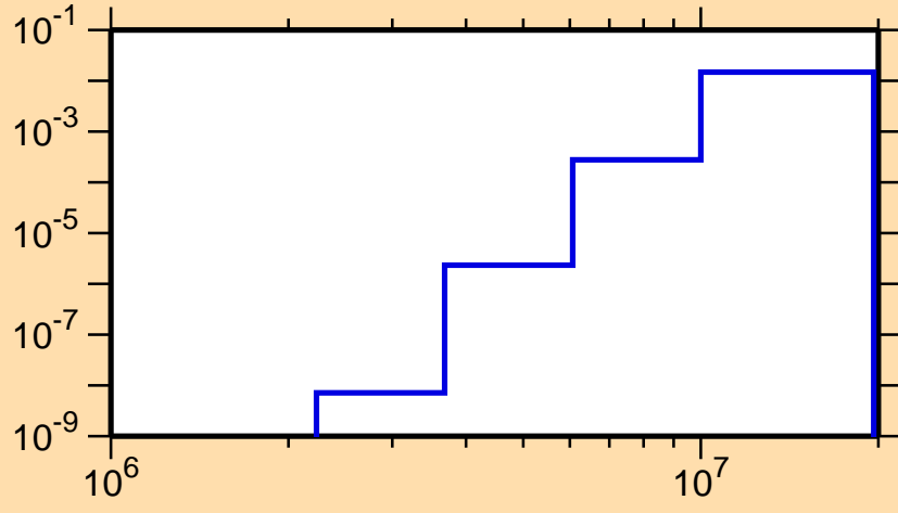
\sigma vs. E for ^{139}\text{Eu}(n,d)
