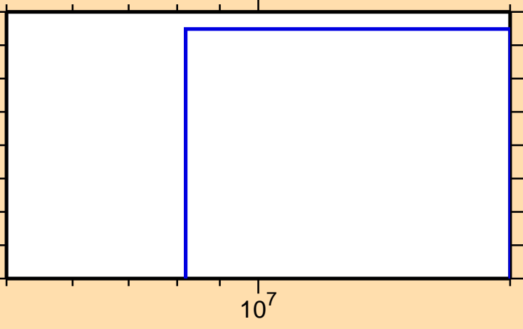
\sigma vs. E for ^{139}\text{Eu}(n,2n\alpha)
