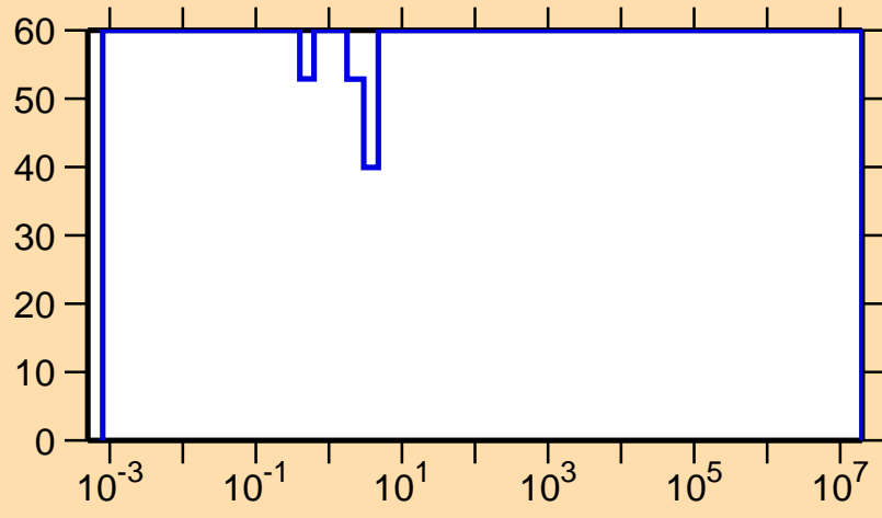
\Delta\sigma/\sigma vs. E for ^{139}\text{Eu}(n,\gamma)
