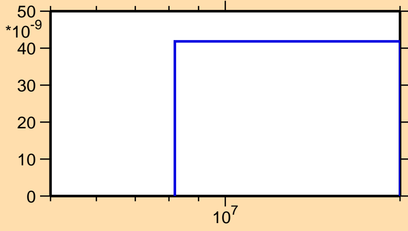
\sigma vs. E for ^{139}\text{Eu}(\text{mt117})
