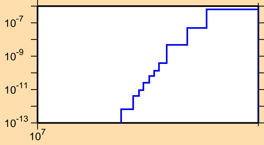
\sigma vs. E for ^{140}\text{Eu}(n,2n\alpha)
