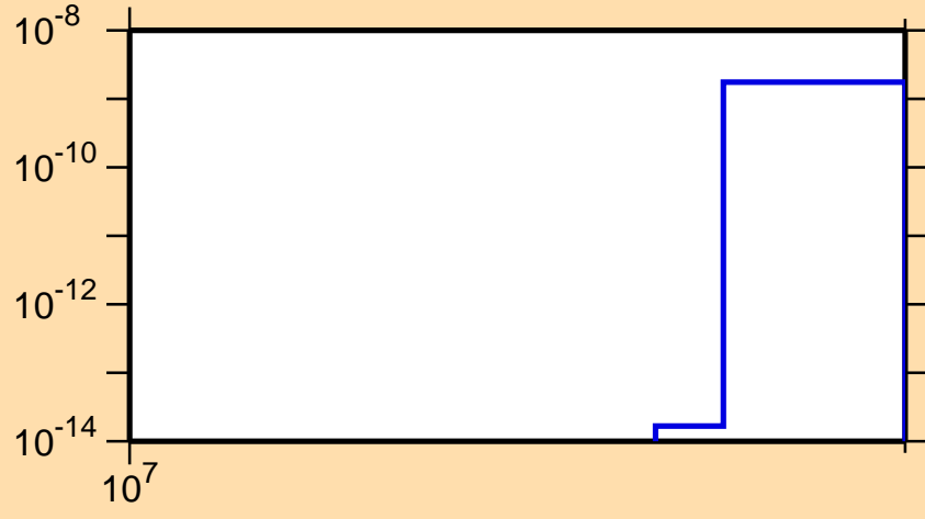
\sigma vs. E for ^{140}\text{Eu}(n,nt)
