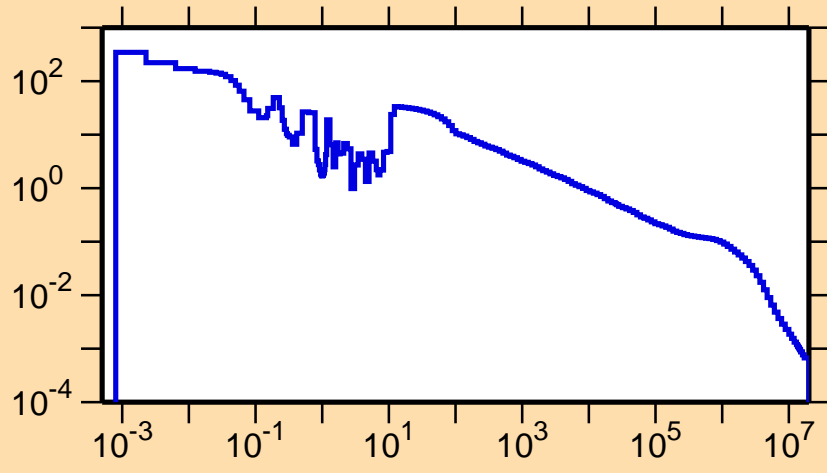
\sigma vs. E for ^{140}\text{Eu}(n,\gamma)
