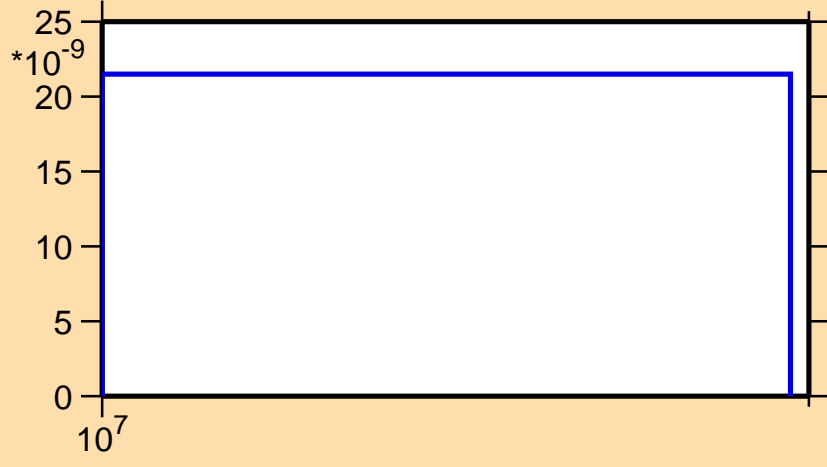
\sigma vs. E for ^{140}\text{Eu}(n,\text{pt})
