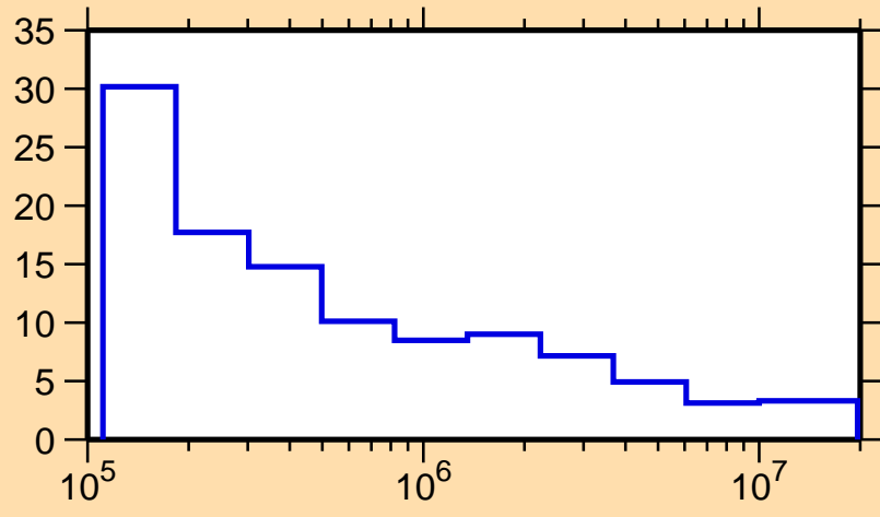
\Delta\sigma/\sigma vs. E for ^{140}\text{Eu}(n,\text{tot.})
