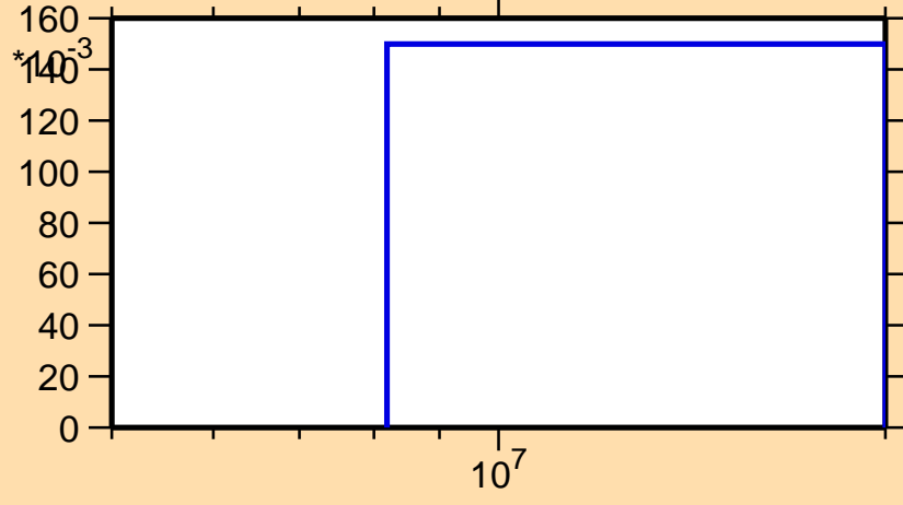
\sigma vs. E for ^{140}\text{Eu}(n,2n)
