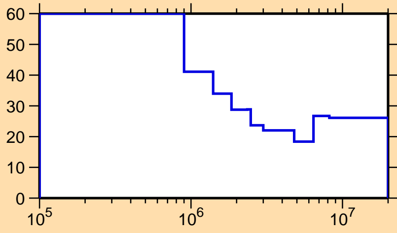
\Delta\sigma/\sigma vs. E for ^{140}\text{Eu}(n,\text{inel.})
