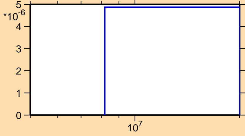
\sigma vs. E for ^{140}\text{Eu}(n,nd)
