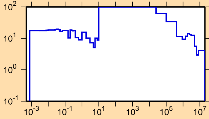
\Delta\sigma/\sigma vs. E for ^{140}\text{Eu}(n,\text{el.})
