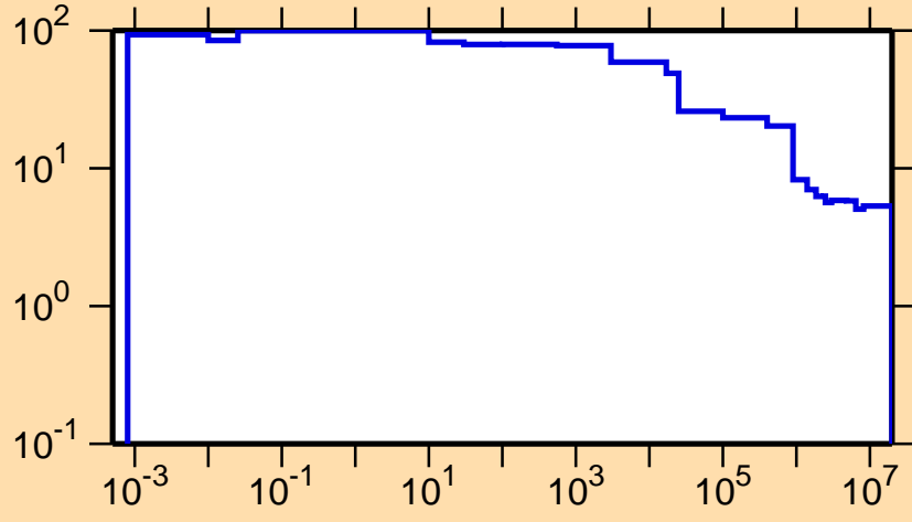
\Delta\sigma/\sigma vs. E for ^{140}\text{Eu}(n,\text{nonel.})
