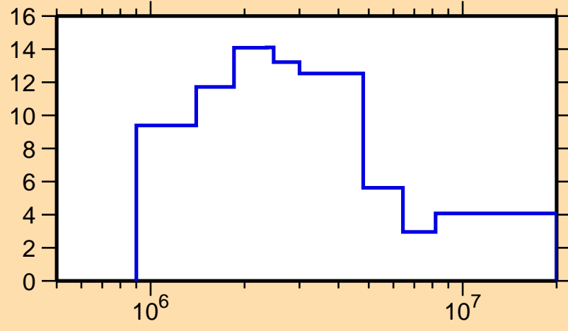
\Delta\sigma/\sigma vs. E for ^{140}\text{Eu}(n,\text{el.})
