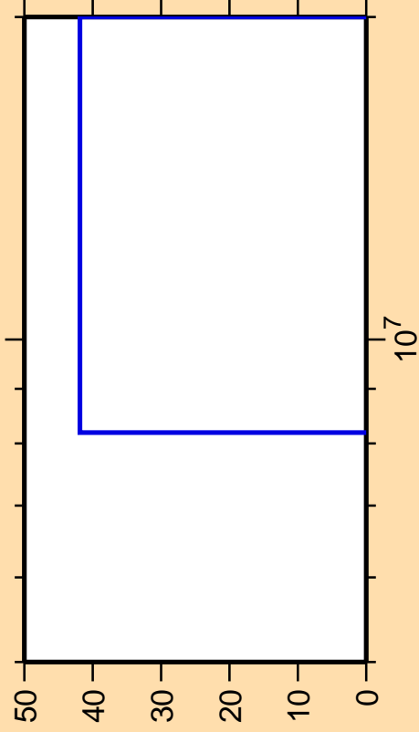
\Delta\sigma/\sigma vs. E for ^{140}\text{Eu}(n,p)
