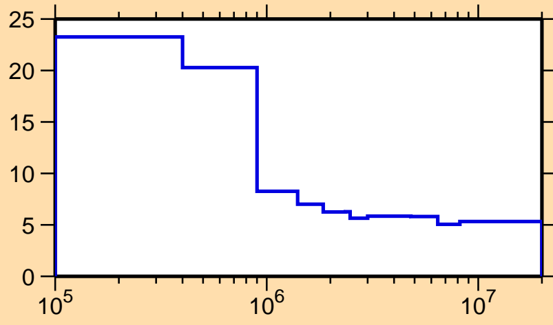
\Delta\sigma/\sigma vs. E for ^{140}\text{Eu}(n,\text{nonel.})
