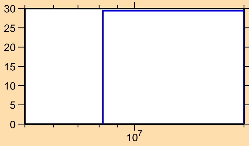
\Delta\sigma/\sigma vs. E for ^{140}\text{Eu}(n,2n)
