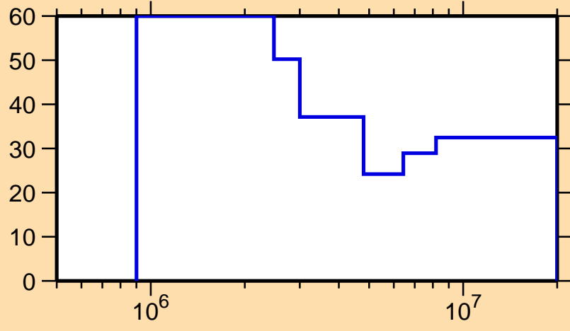
\Delta\sigma/\sigma vs. E for ^{140}\text{Eu}(n,n\text{cont.})
