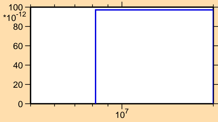
\sigma vs. E for ^{140}\text{Eu}(\text{mt } 34)
