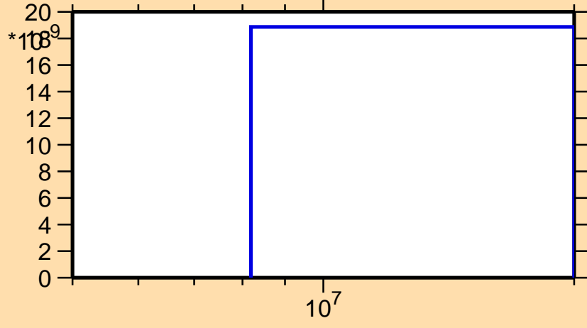
\sigma vs. E for ^{140}\text{Eu}(\text{mt117})
