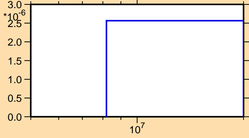
\sigma vs. E for ^{140}\text{Eu}(n,\text{pd})
