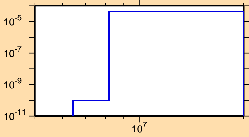
\sigma vs. E for ^{140}\text{Eu}(n,\text{He3})
