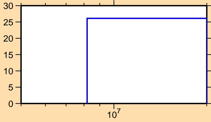
\Delta\sigma/\sigma vs. E for ^{140}\text{Eu}(n,\text{inel.})
