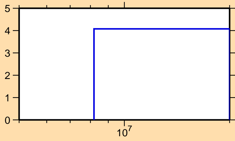
\Delta\sigma/\sigma vs. E for ^{140}\text{Eu}(n,\text{el.})
