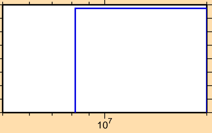
\sigma vs. E for ^{140}\text{Eu}(n,2n\alpha)
