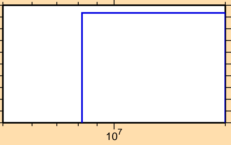
\sigma vs. E for ^{140}\text{Eu}(n,\text{pt})
