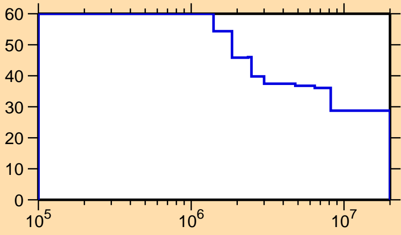
\Delta\sigma/\sigma vs. E for ^{140}\text{Eu}(n,n_1)
