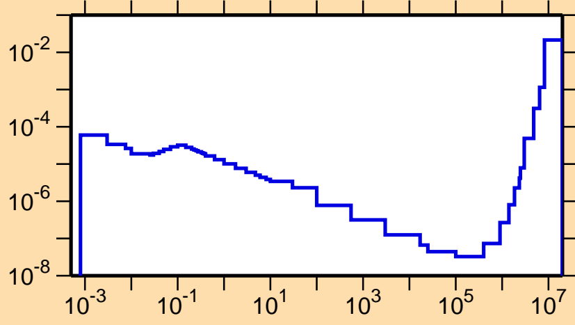
\sigma vs. E for ^{140}\text{Eu}(n,p\alpha)
