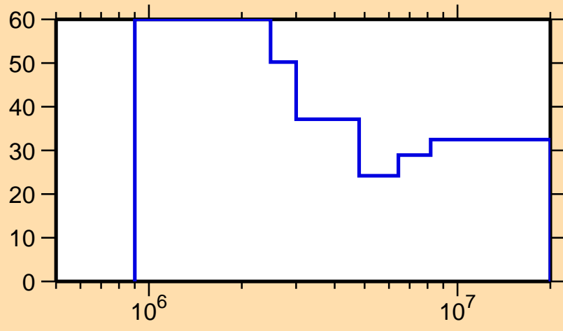
\Delta\sigma/\sigma vs. E for ^{140}\text{Eu}(n,n\text{cont.})
