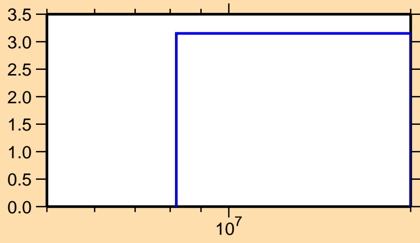
\Delta\sigma/\sigma vs. E for ^{140}\text{Eu}(n,\text{tot.})
