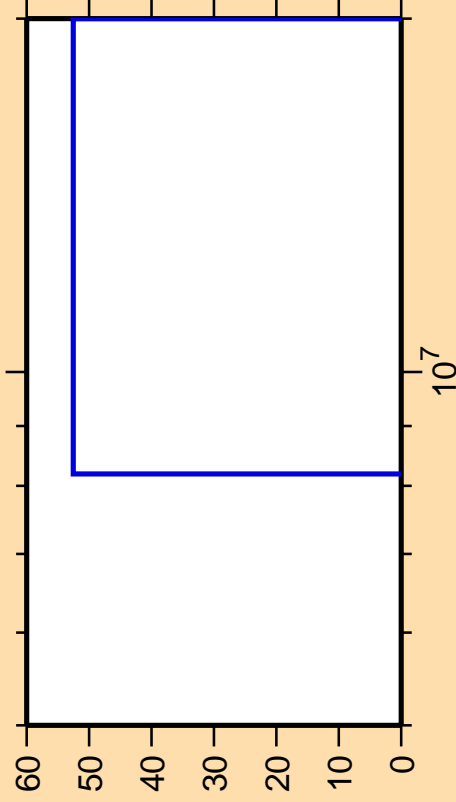
\Delta\sigma/\sigma vs. E for ^{140}\text{Eu}(n,2np)
