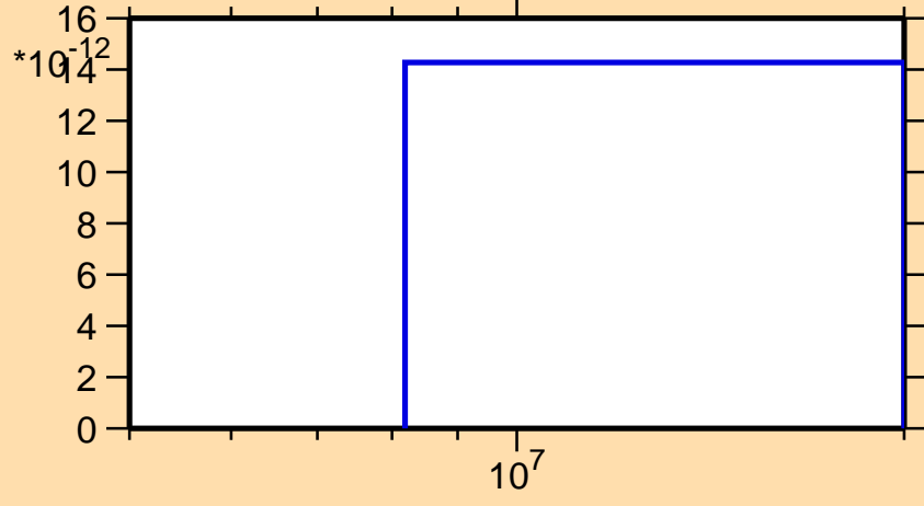
\sigma vs. E for ^{140}\text{Eu}(n,nt)
