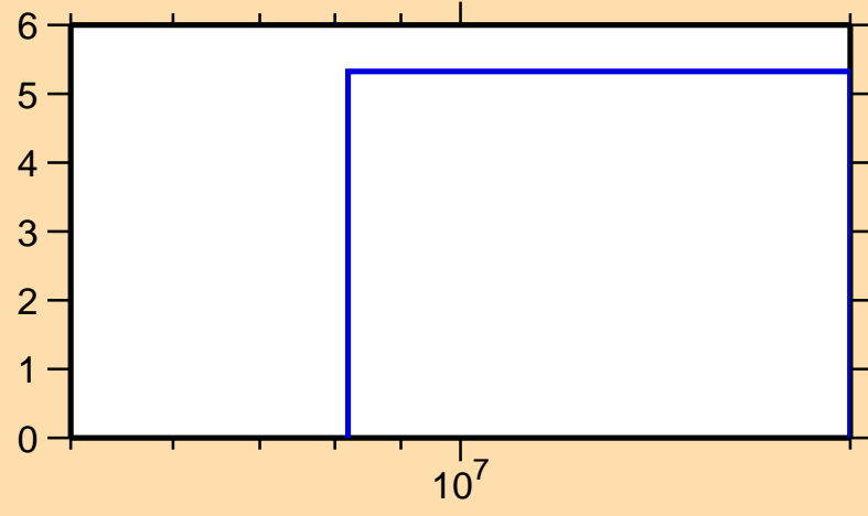
\Delta\sigma/\sigma vs. E for ^{140}\text{Eu}(n,\text{nonel.})
