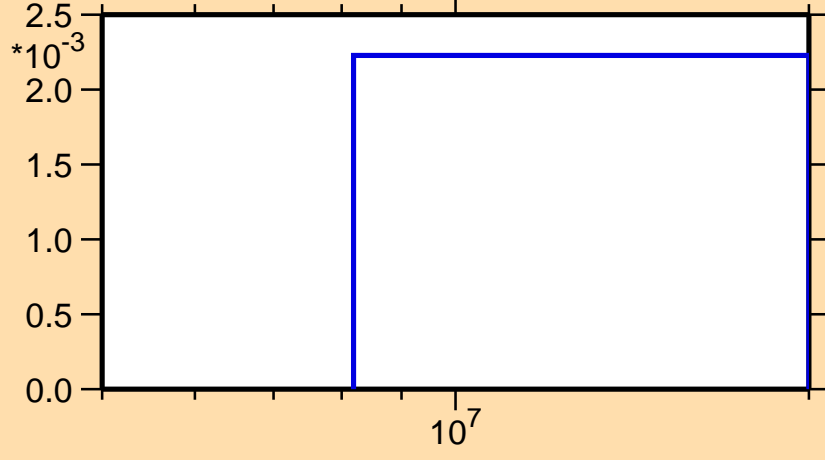
\sigma vs. E for ^{140}\text{Eu}(n,2np)
