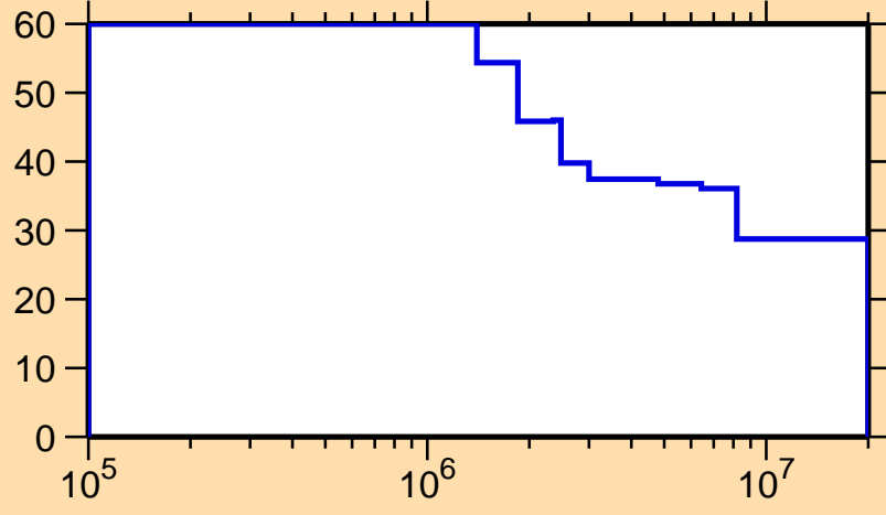
\Delta\sigma/\sigma vs. E for ^{140}\text{Eu}(n,n_1)
