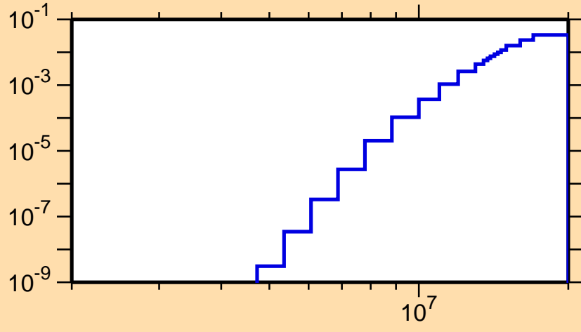
\sigma vs. E for ^{141}\text{Eu}(n,n\alpha)
