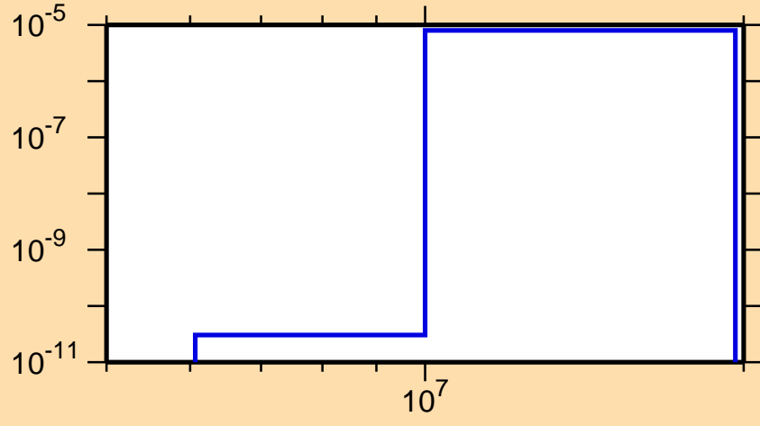
\sigma vs. E for ^{141}\text{Eu}(n,\text{He3})
