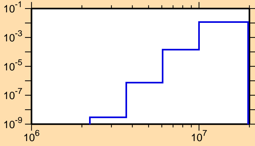
\sigma vs. E for ^{141}\text{Eu}(n,d)
