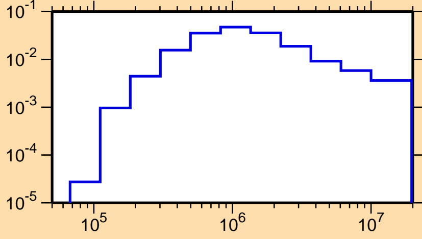
\sigma vs. E for ^{141}\text{Eu}(n,n_1)
