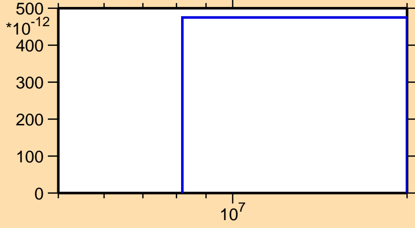
\sigma vs. E for ^{141}\text{Eu}(n,2n\alpha)
