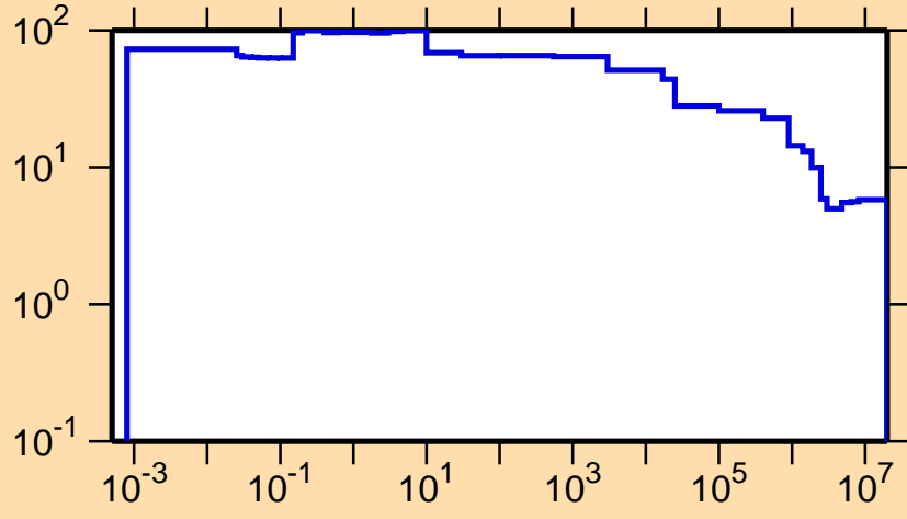
\Delta\sigma/\sigma vs. E for ^{141}\text{Eu}(n,\text{nonel.})
