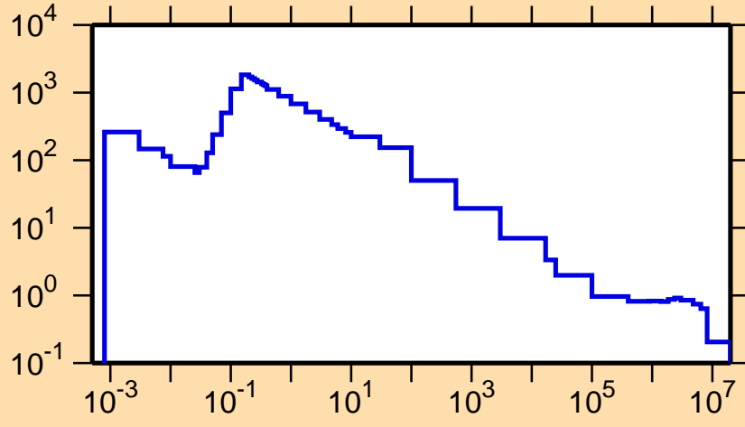
\sigma vs. E for ^{141}\text{Eu}(n,p)
