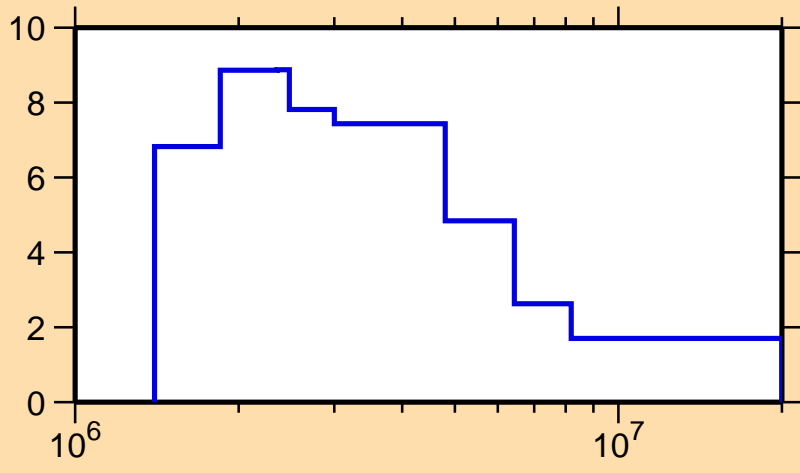
\Delta\sigma/\sigma vs. E for ^{141}\text{Eu}(n,\text{tot.})
