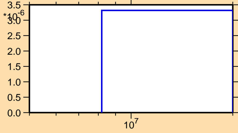
\sigma vs. E for ^{141}\text{Eu} (mt 45)
