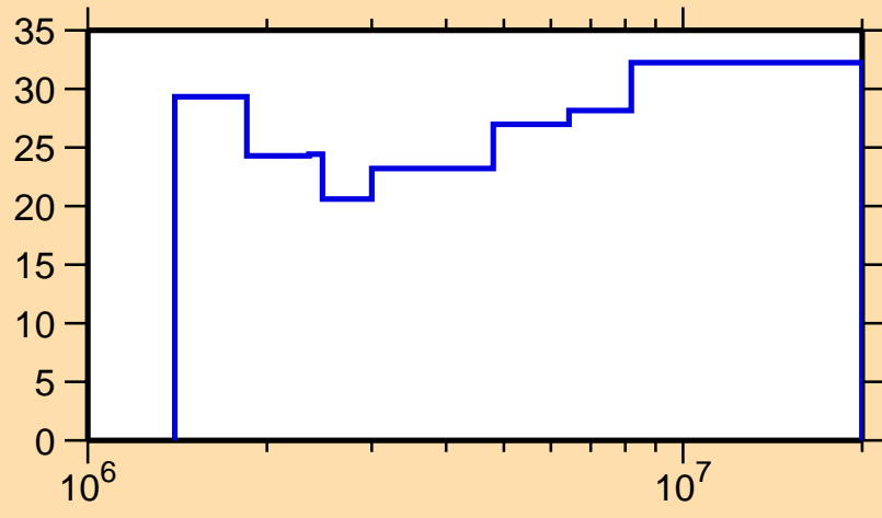
\Delta\sigma/\sigma vs. E for ^{141}\text{Eu}(n,n_1)
