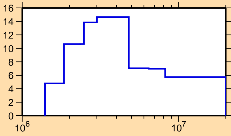
\Delta\sigma/\sigma vs. E for ^{141}\text{Eu}(n,\text{el.})
