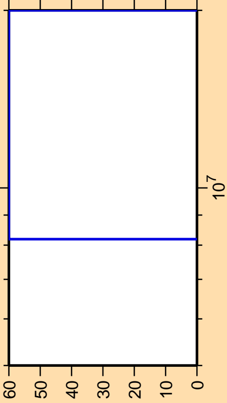
\Delta\sigma/\sigma vs. E for ^{141}\text{Eu}(n,2np)
