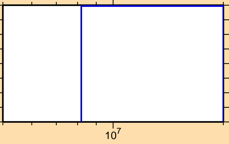
\sigma vs. E for ^{141}\text{Eu}(n,nt)
