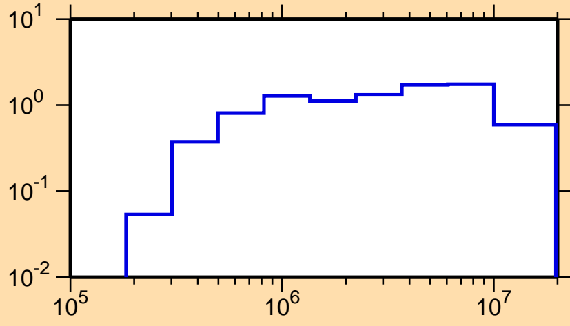
\sigma vs. E for ^{142}\text{Eu}(n,\text{inel.})
