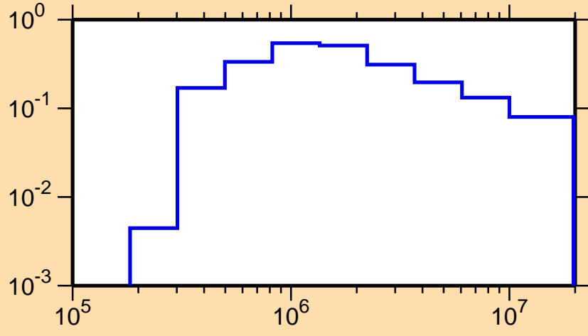
\sigma vs. E for ^{142}\text{Eu}(n,n_3)
