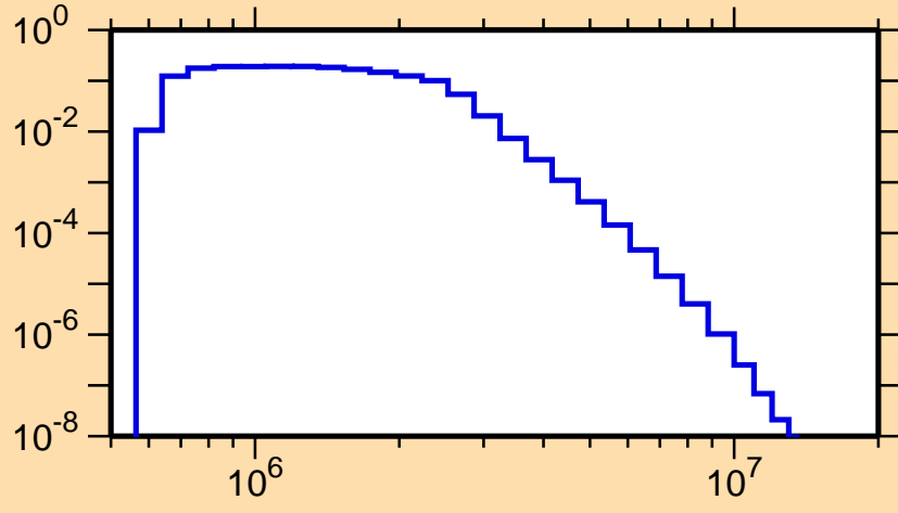
\sigma vs. E for ^{144}\text{Eu}(n,n_4)
