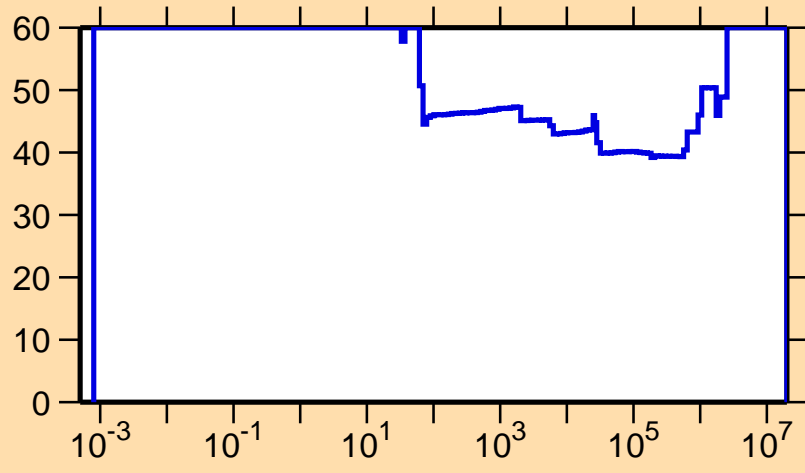
\Delta\sigma/\sigma vs. E for ^{144}\text{Eu}(n,\gamma)
