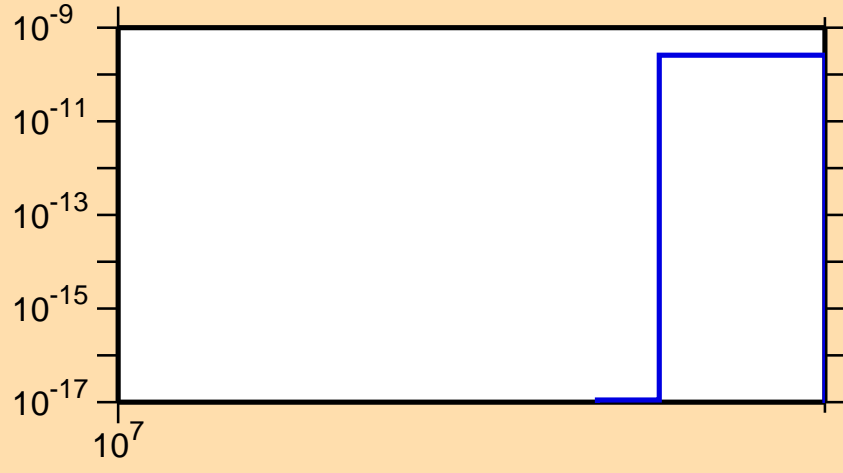
\sigma vs. E for ^{144}\text{Eu}(n,nt)
