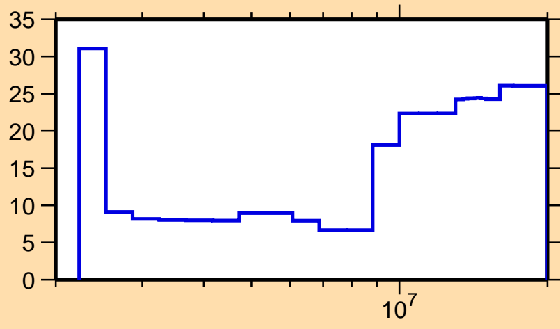
\Delta\sigma/\sigma vs. E for ^{144}\text{Eu}(n,n\text{cont.})
