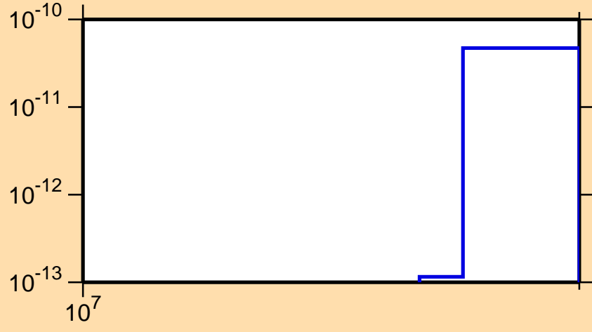
\sigma vs. E for ^{144}\text{Eu} (mt 34)
