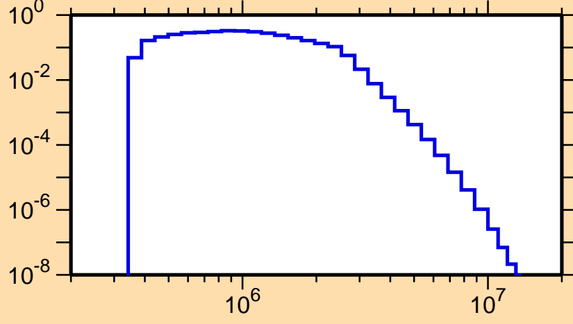
\sigma vs. E for ^{144}\text{Eu}(n,n_2)
