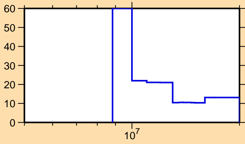
\Delta\sigma/\sigma vs. E for ^{144}\text{Eu}(n,2n)
