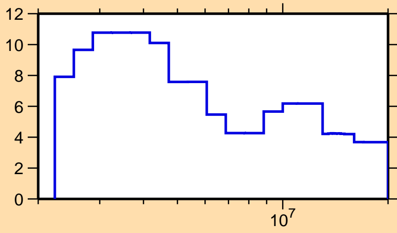
\Delta\sigma/\sigma vs. E for ^{144}\text{Eu}(n,\text{el.})
