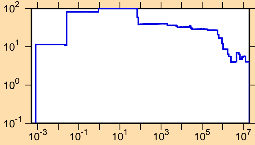
\Delta\sigma/\sigma vs. E for ^{144}\text{Eu}(n,\text{nonel.})
