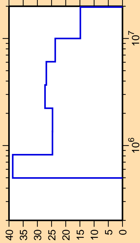
\Delta\sigma/\sigma vs. E for ^{144}\text{Eu}(n,n_3)
