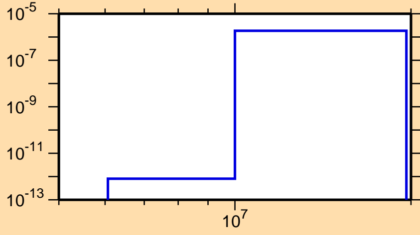
\sigma vs. E for ^{144}\text{Eu}(n,\text{He3})
