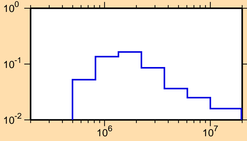
\sigma vs. E for ^{144}\text{Eu}(n,n_3)
