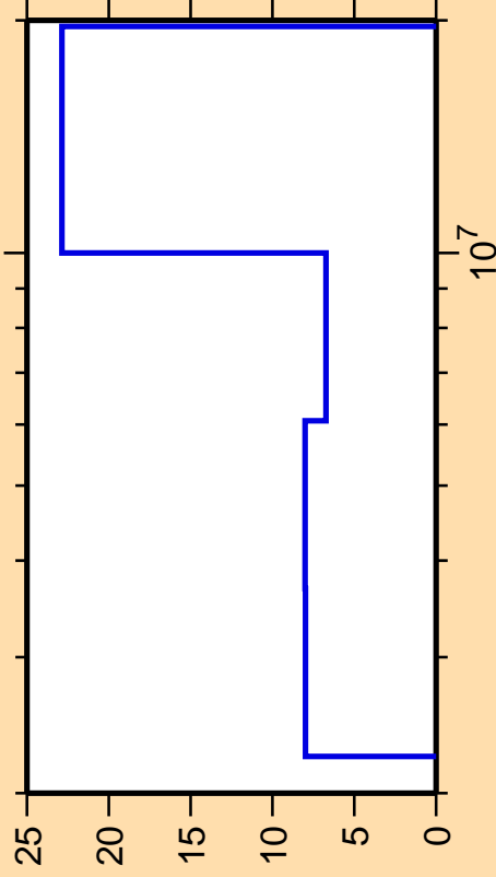
\Delta\sigma/\sigma vs. E for ^{144}\text{Eu}(n,n\text{cont.})
