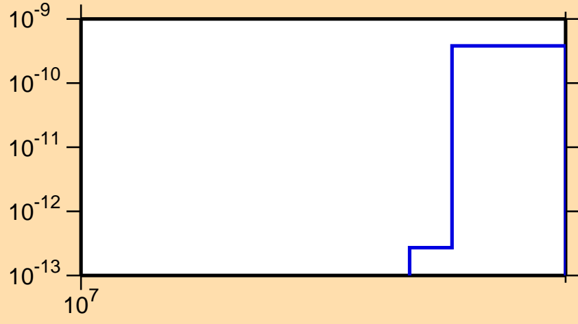
\sigma vs. E for ^{145}\text{Eu}(n,2n\alpha)
