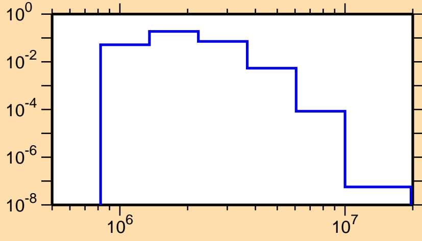
\sigma vs. E for ^{145}\text{Eu}(n,n_4)
