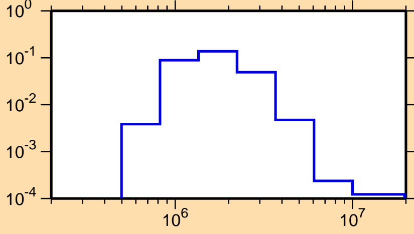
\sigma vs. E for ^{145}\text{Eu}(n,n_2)
