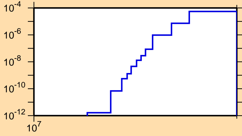
\sigma vs. E for ^{147}\text{Eu}(n,nd)
